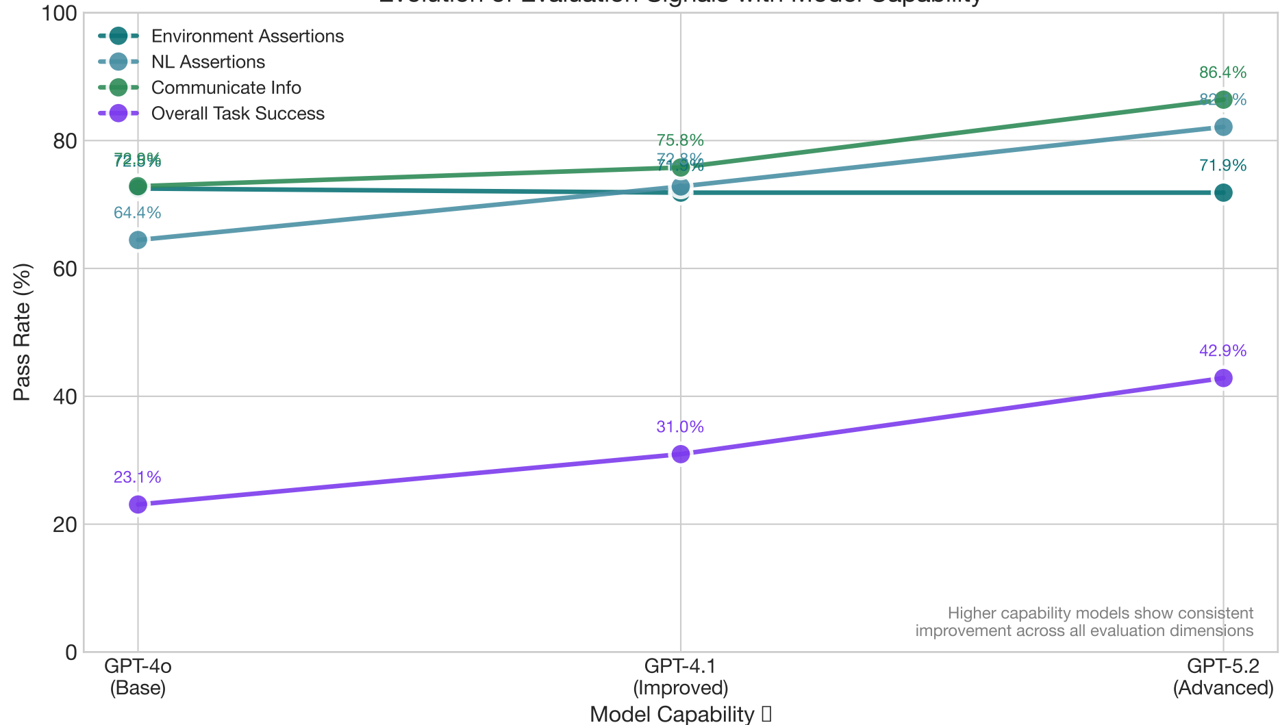
Evolution of Evaluation Signals with Model Capability
