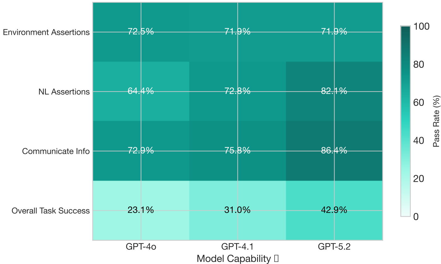
Evaluation Signal Pass Rates Across Models
