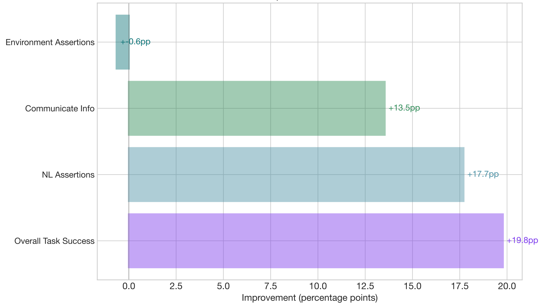
Performance Improvement: GPT-4o □ GPT-5.2
