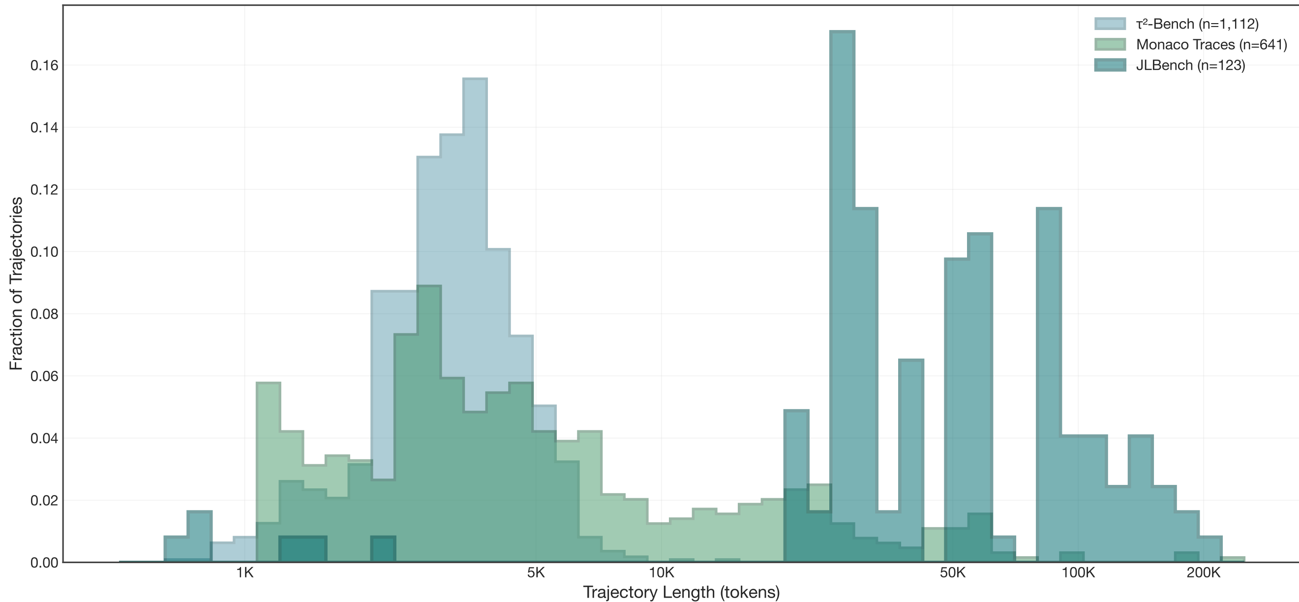
Trajectory Length Distribution Comparison
