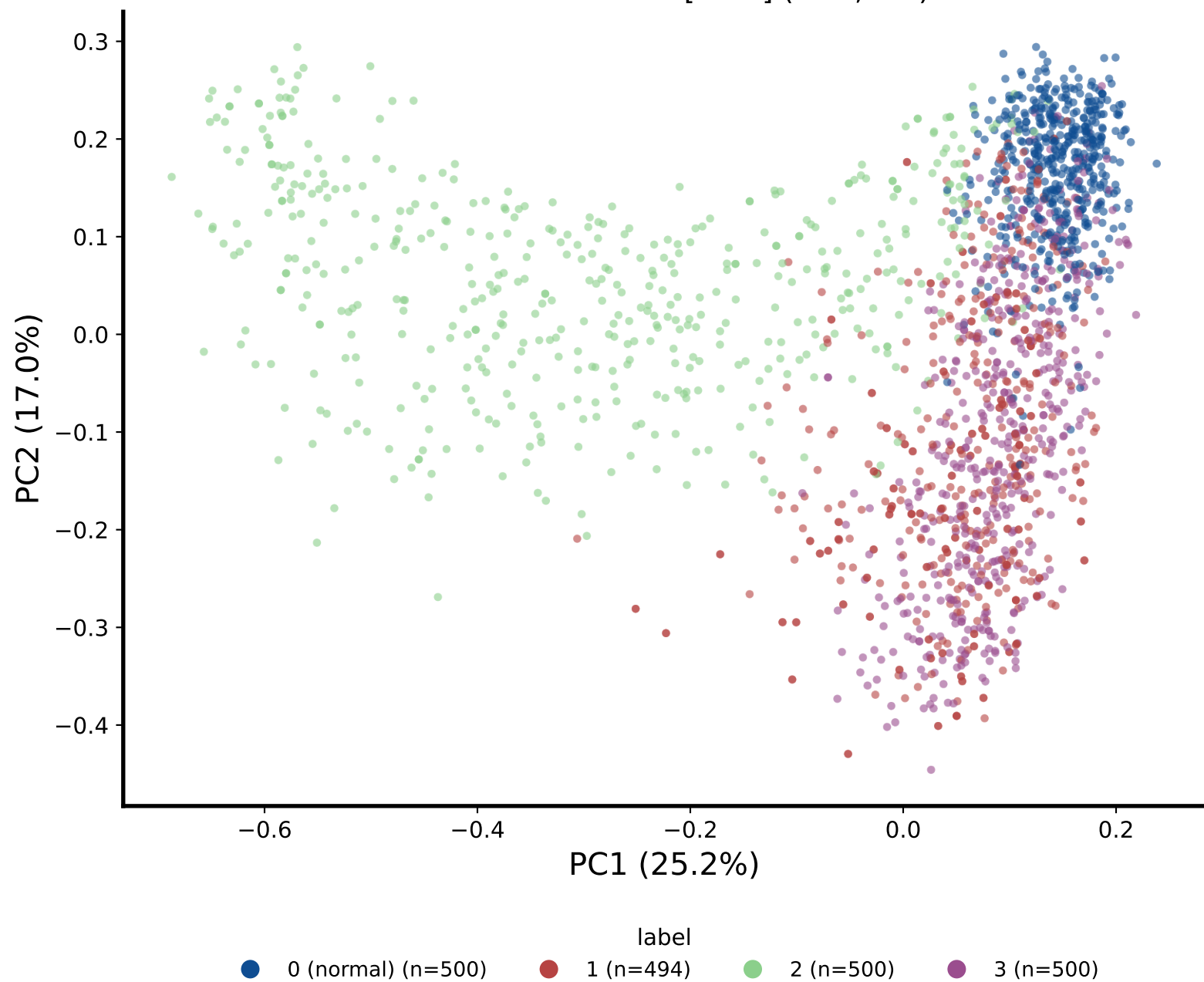
Fundus · BiomedCLIP AMDNet23 Dataset [train] (n=1,994)
