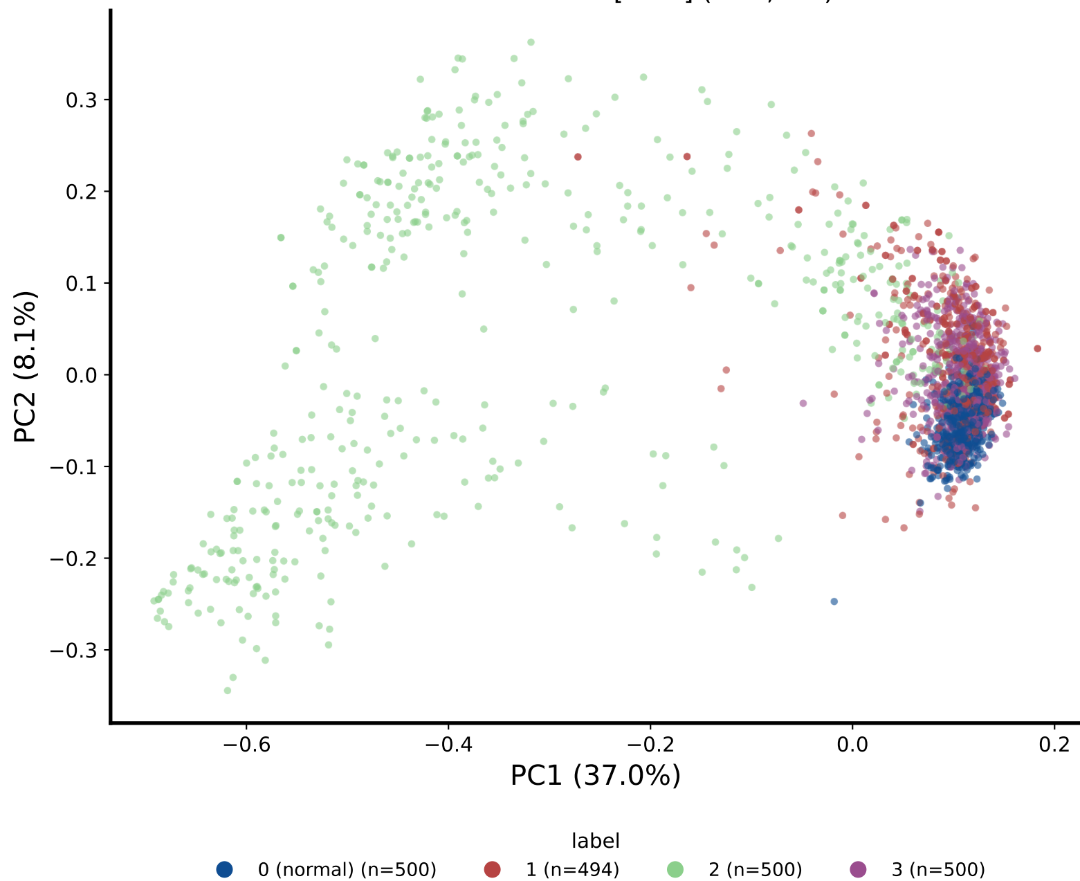
Fundus · CLIP AMDNet23 Dataset [train] (n=1,994)
