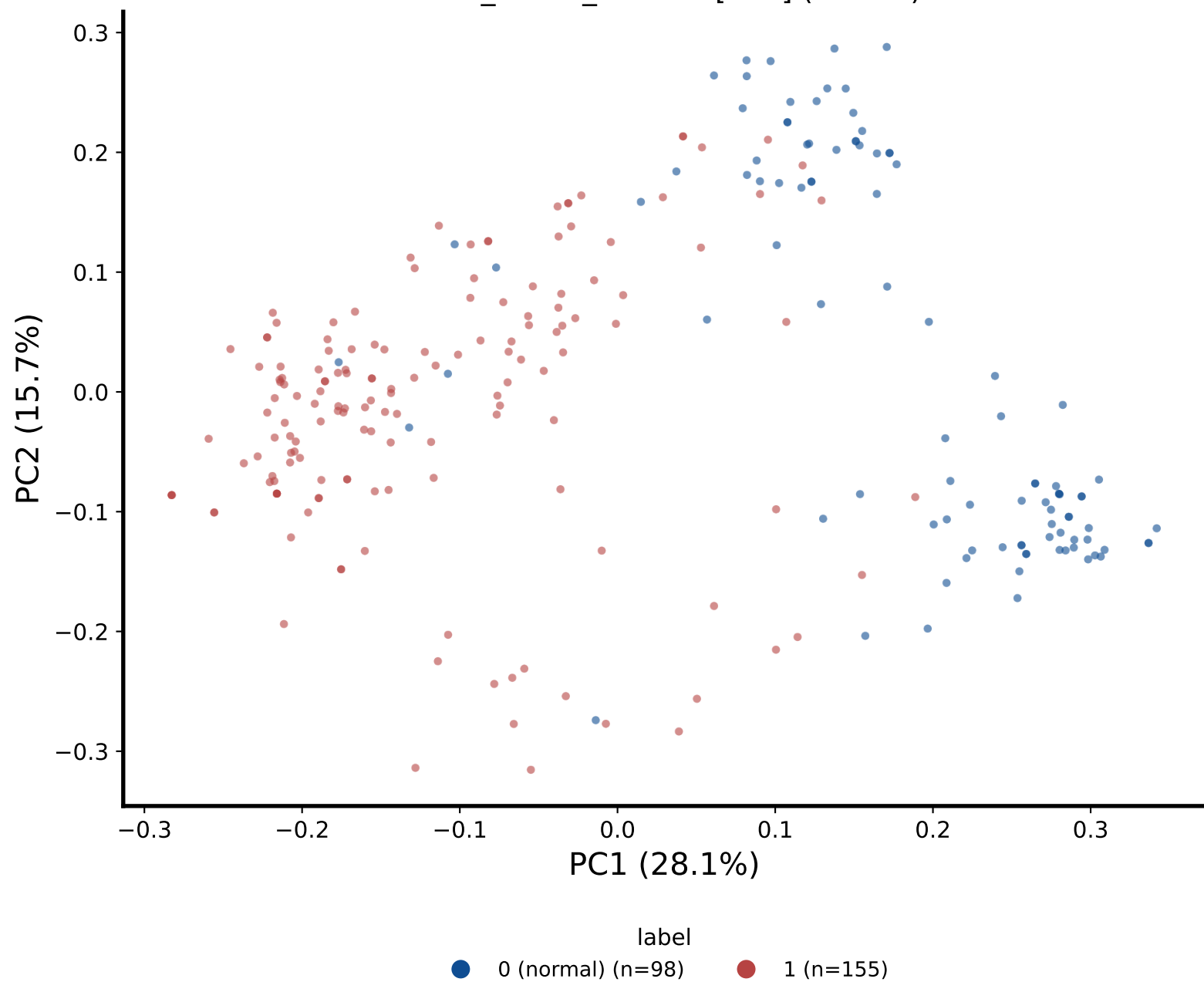
MRI · CLIP brain_tumor_dataset [test] (n=253)
