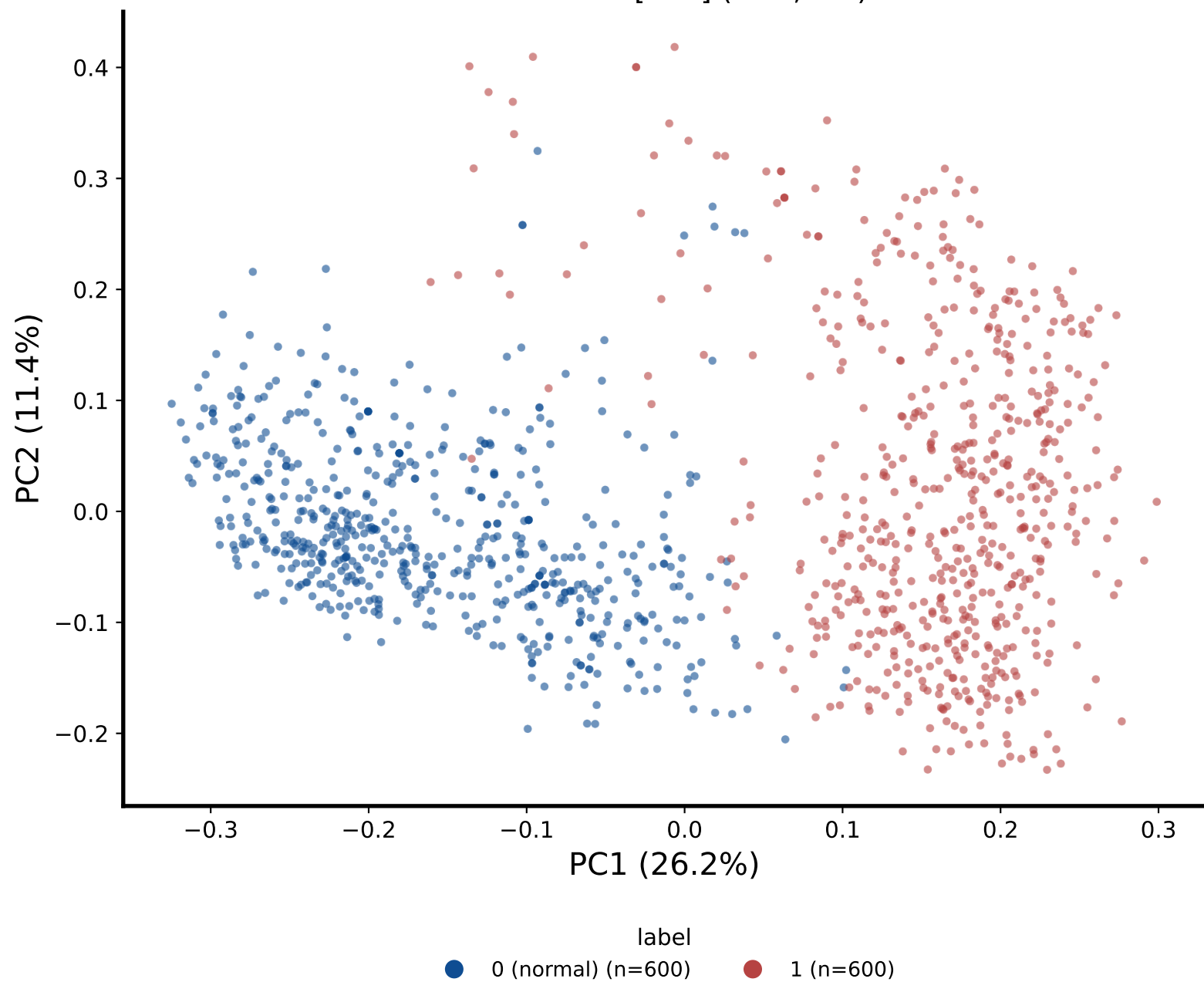
MRI · CLIP BrainTumor [test] (n=1,200)
