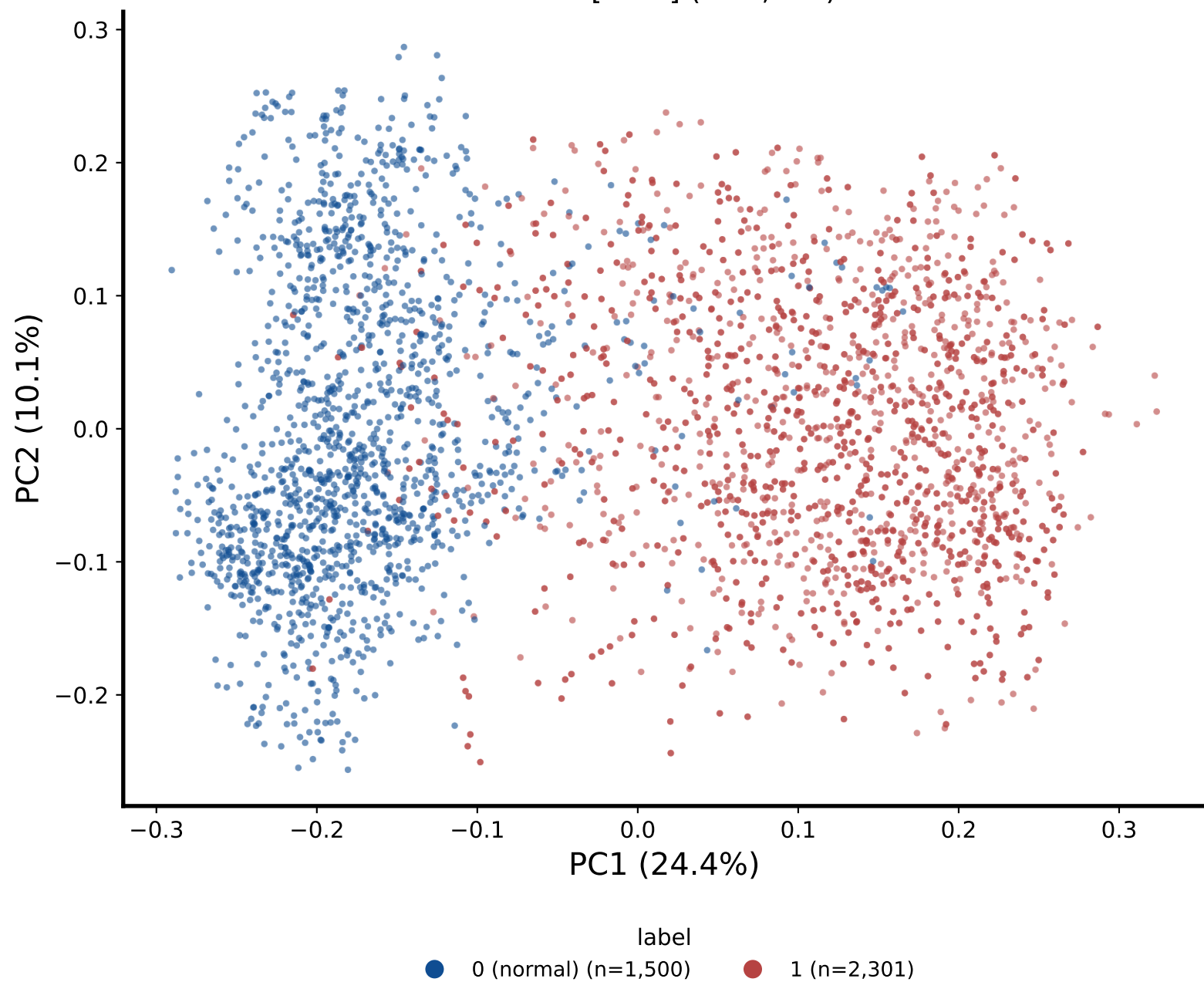
MRI · CLIP Br35H [train] (n=3,801)
