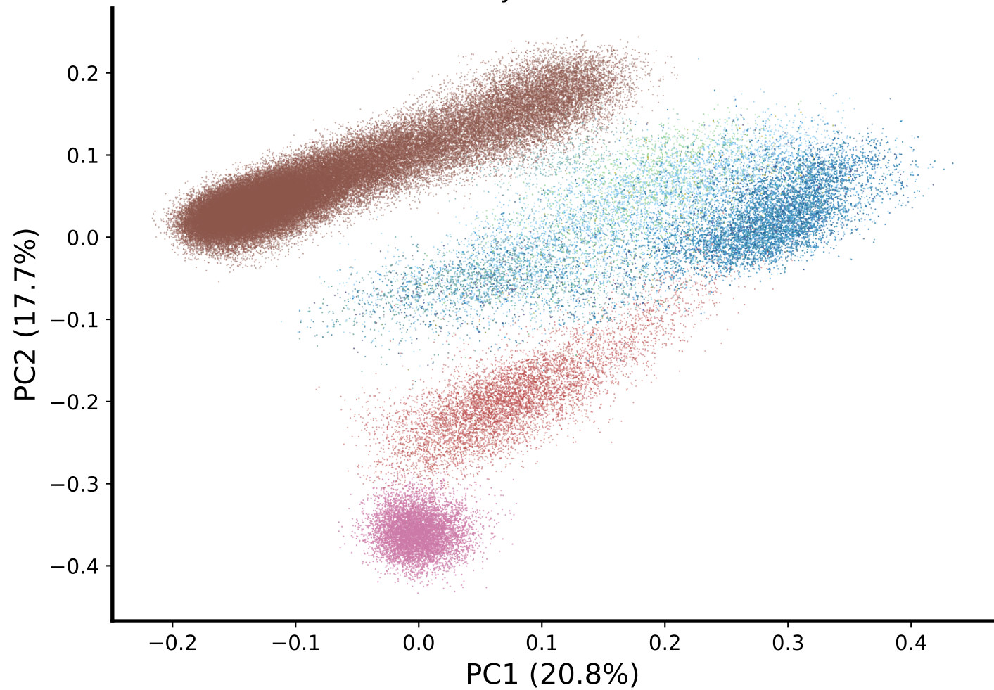
By dataset
