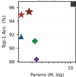
CIFAR-10
