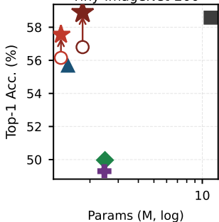
Tiny-ImageNet-200
