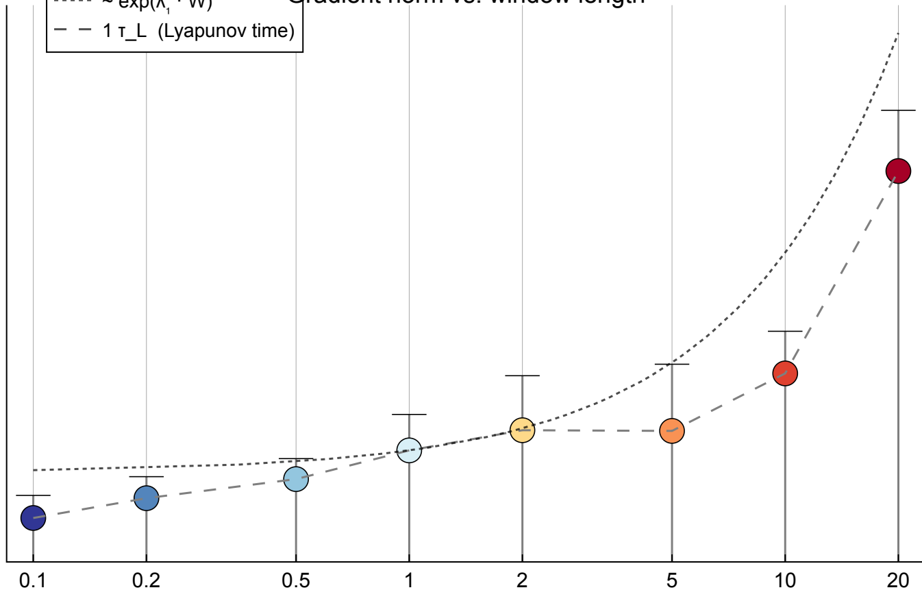
Gradient norm vs. window length
