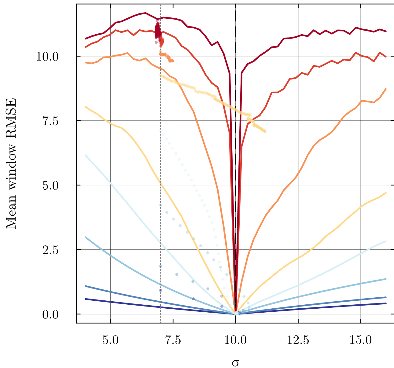
Loss landscape — \sigma slice ( \rho=28, \beta=8/3 fixed)
