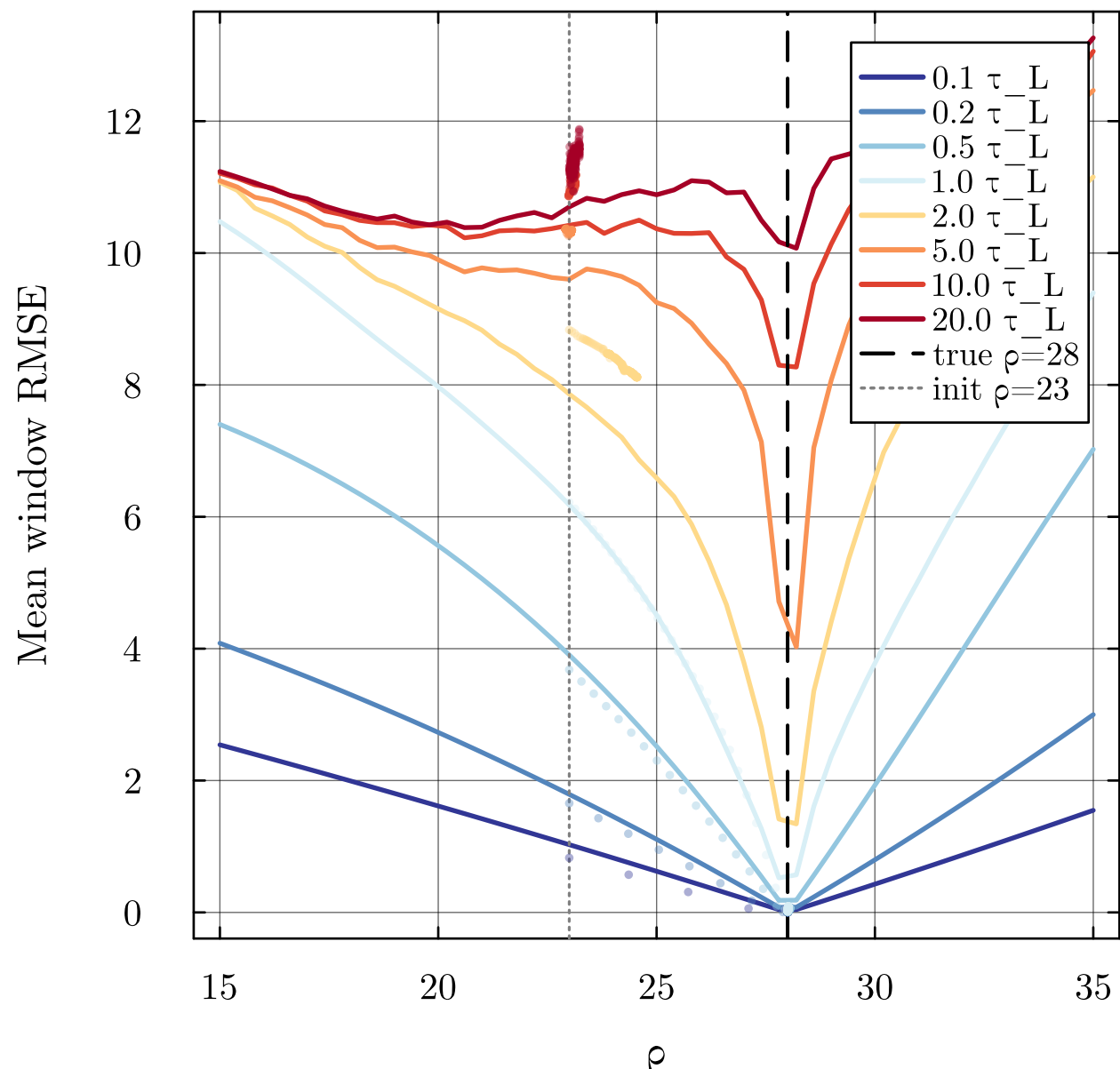
Loss landscape — \rho slice ( \sigma=10, \beta=8/3 fixed)
