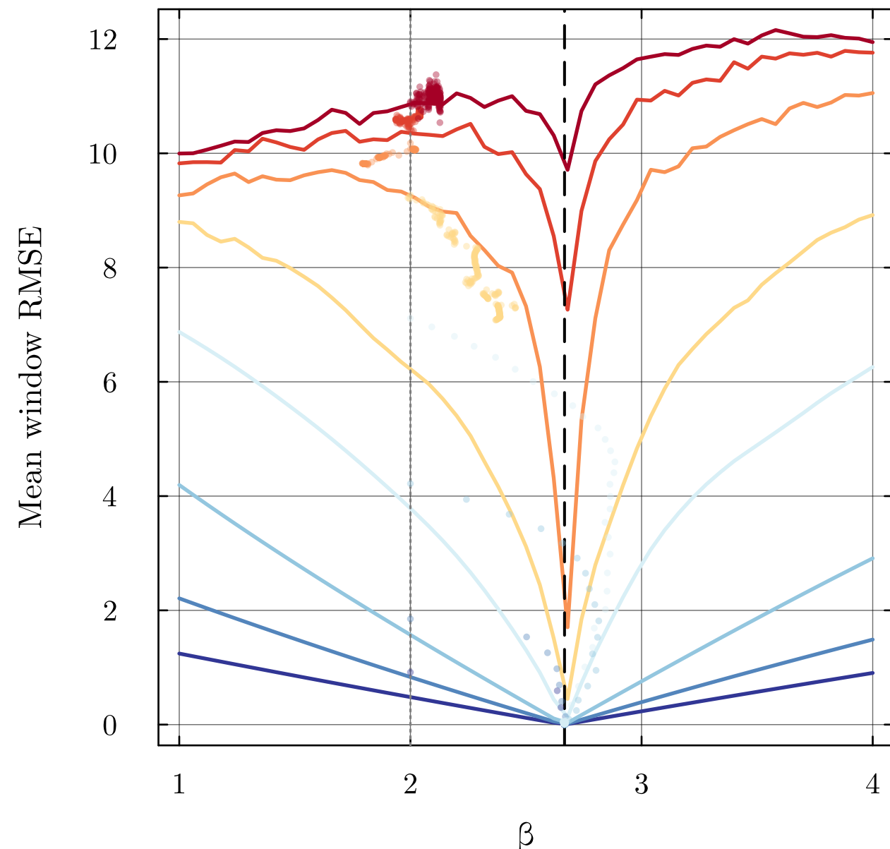
Loss landscape — \beta slice ( \sigma=10, \rho=28 fixed)
