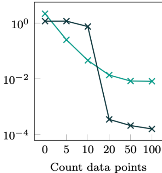
2D nonlinear
