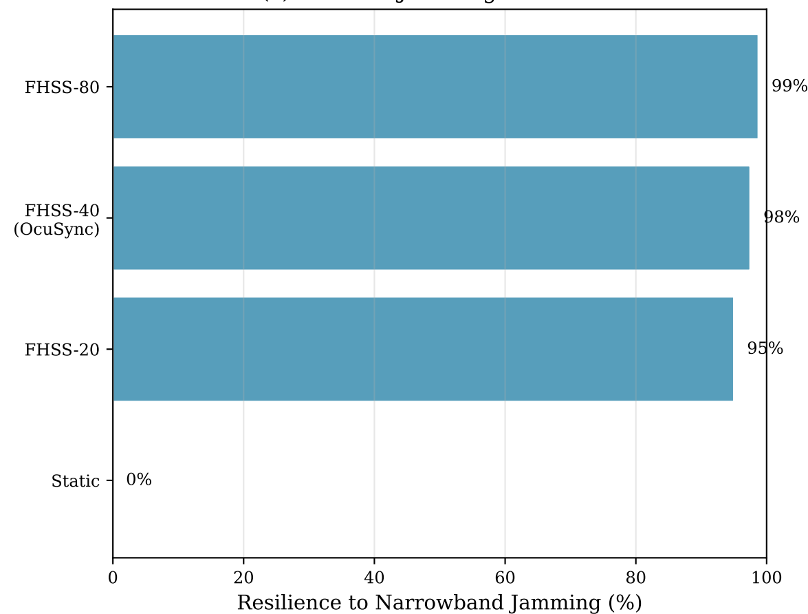
(c) Protocol Jamming Resilience
