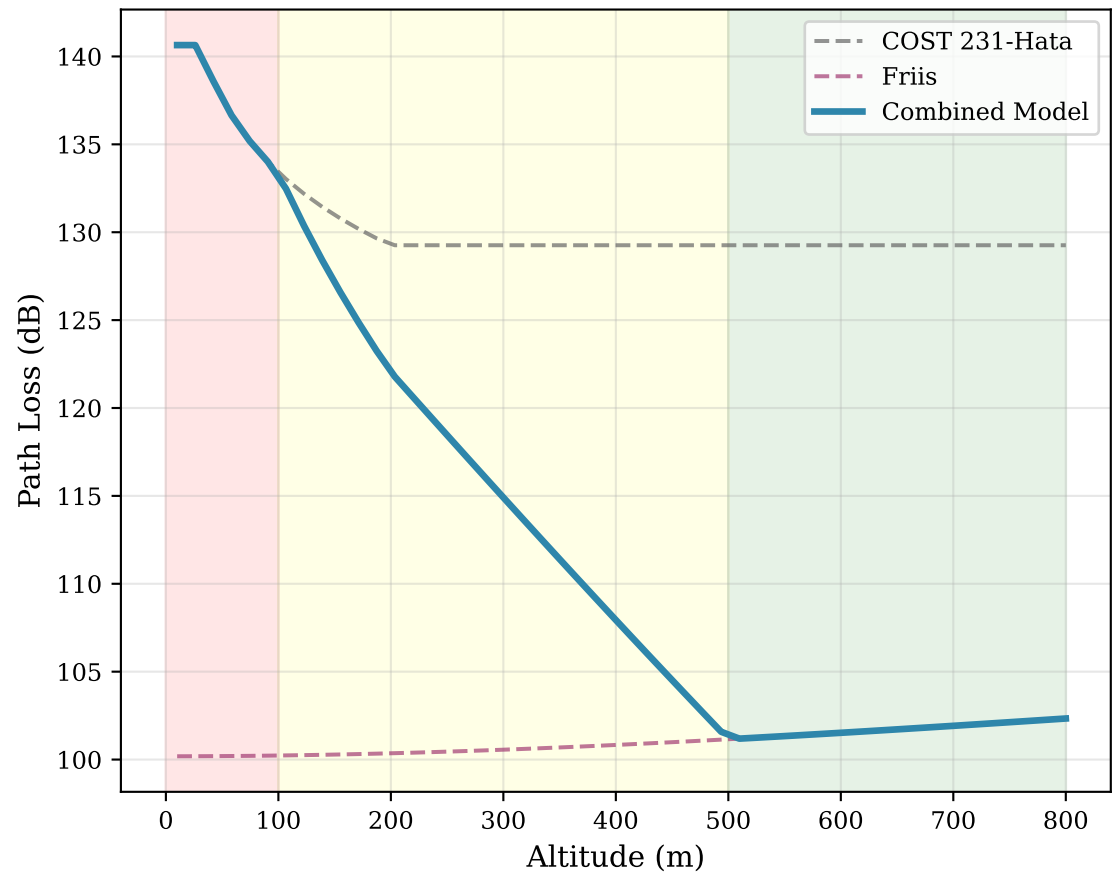
(b) Path Loss vs Altitude ( d = 1000\text{m} )
