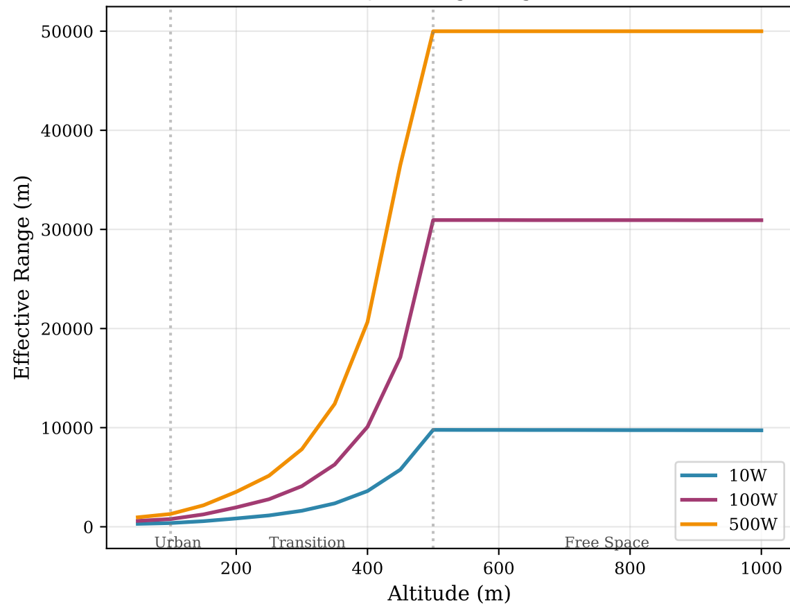
(a) Effective Jamming Range vs Altitude
