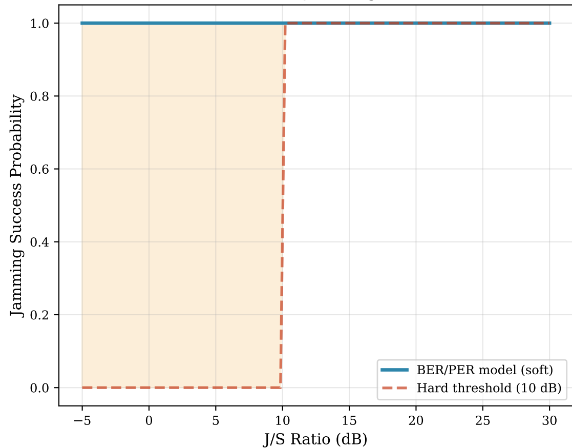
(b) Soft vs Hard Jamming Threshold
