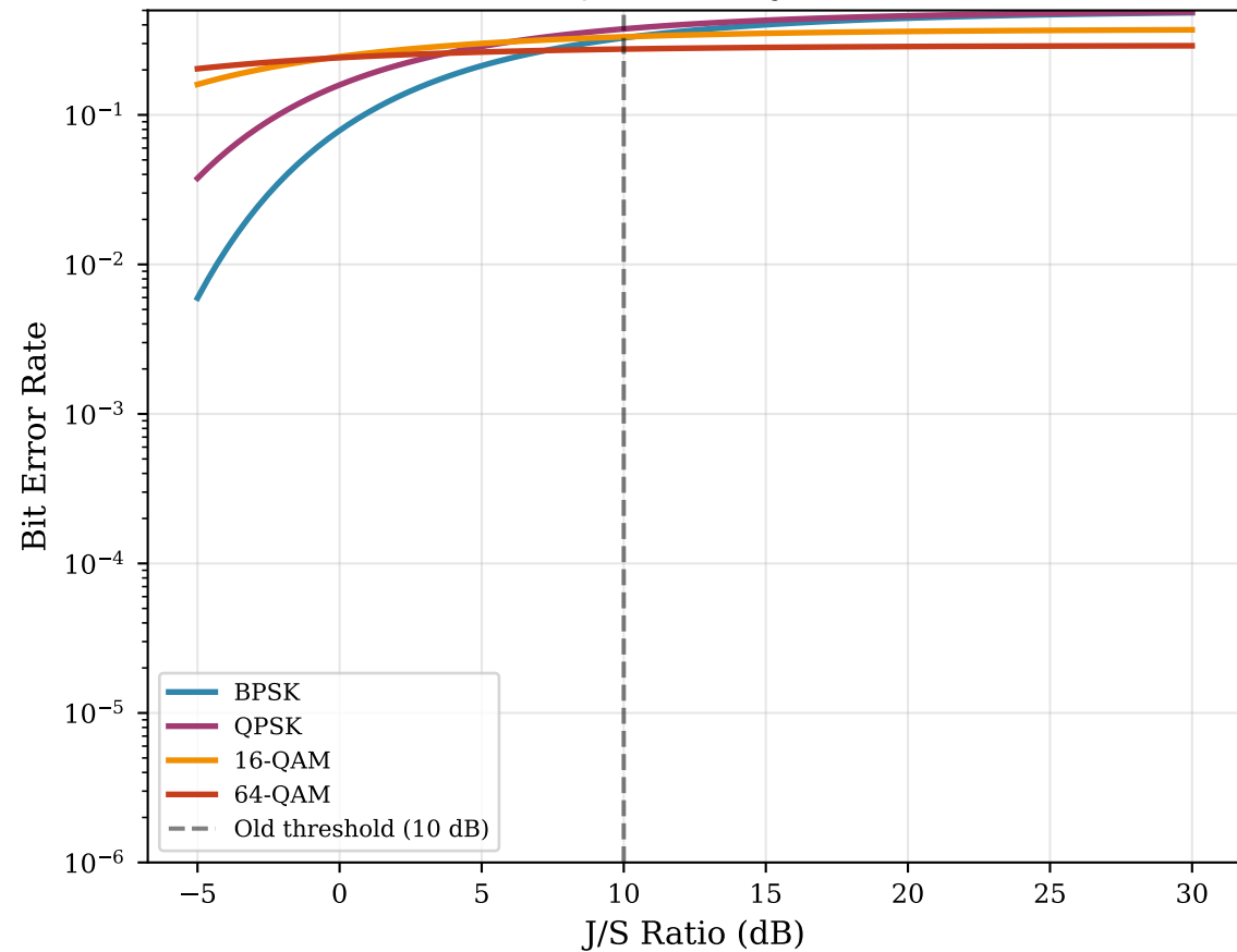
(a) BER vs J/S Ratio by Modulation
