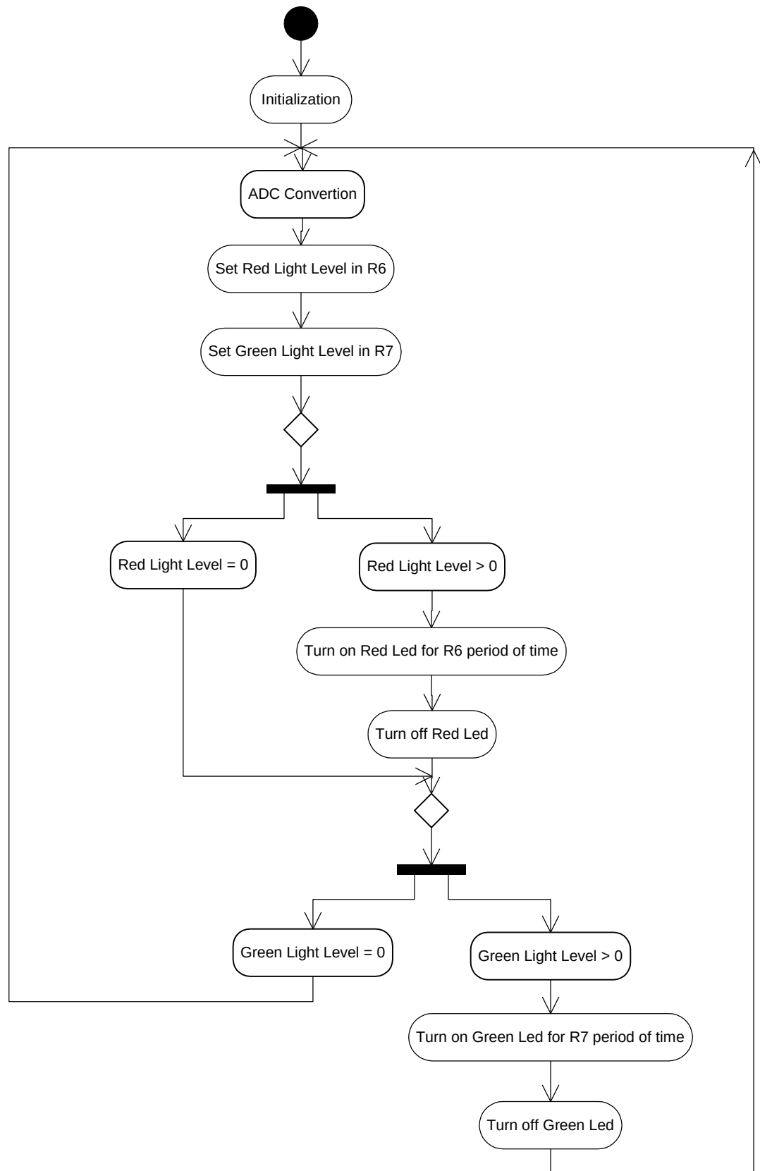
Fig. 3.2.2. RedGreenLed algorithm
