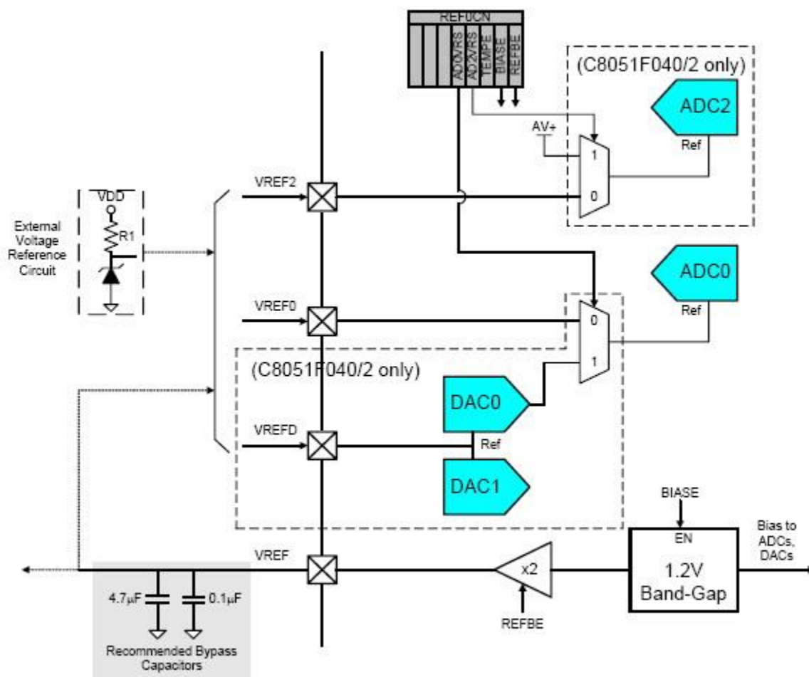
Fig. 2.1.3. Voltage Reference block diagram
