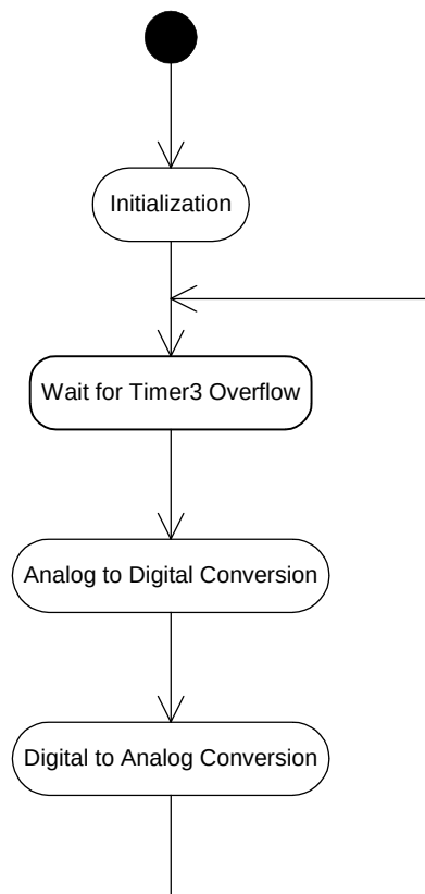
Fig. 3.2.2.b. Organigrama aplicatiei AD-DAConversion_v2
