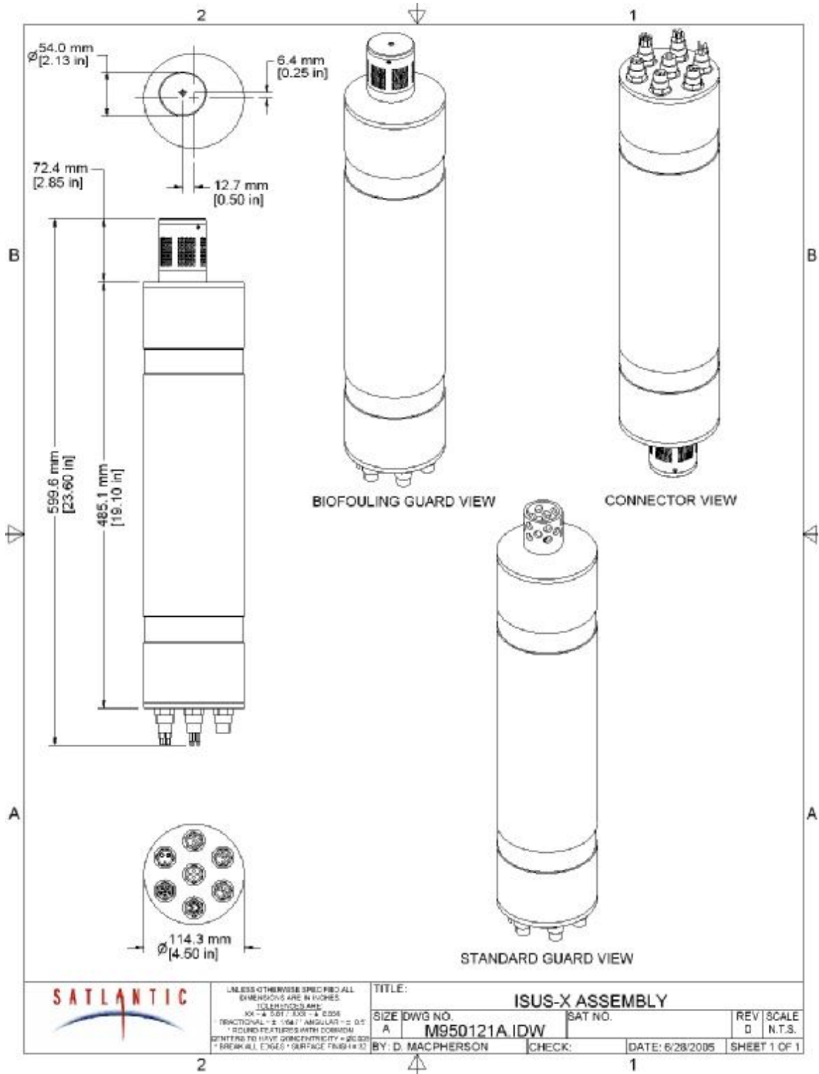
Figure A-4: The MBARI-ISUS-X v.2 Anodized Aluminum Body
