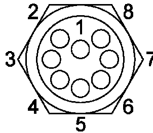
Figure A-11: MCBH8F Bulkhead, Female Face View
