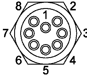
Figure A-9: MCBH8M Bulkhead, Male Face View
