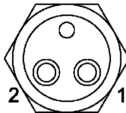
Figure A-6: MCBH2M Bulkhead, Male Face View
