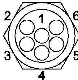
Figure A-10: MCBH6F Bulkhead, Female Face View
