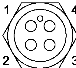
Figure A-8: MCBH4F Bulkhead, Female Face View
