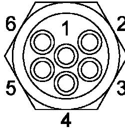
Figure A-7: MCBH6M Bulkhead, Male Face View
