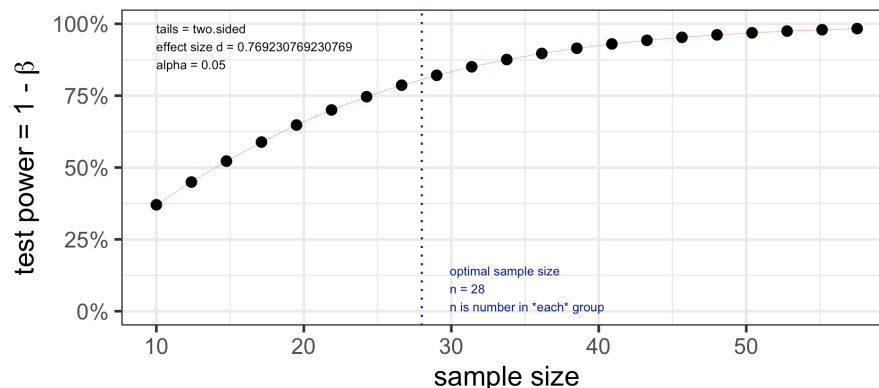
Two-sample t test power calculation
