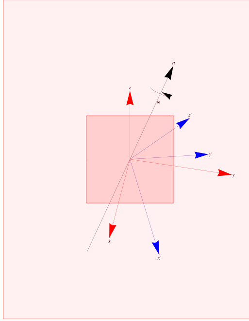
Figure 1.6. Rotation of a coordinate system through an angle \omega about an axis \mathbf{n}(\Theta, \Phi) .
