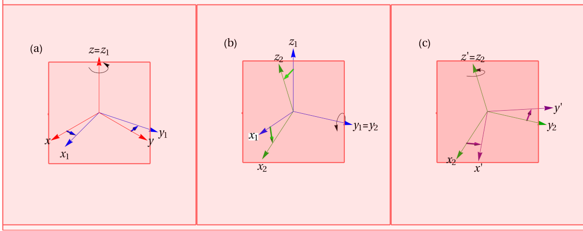
Figure 1.3. Succession of rotations of a coordinate system according to scheme A.
