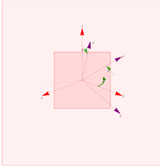
Figure 1.5. The Euler angles \alpha, \beta, \gamma .
