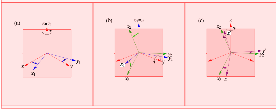
Figure 1.4. Succession of rotations of a coordinate system according to scheme B.
