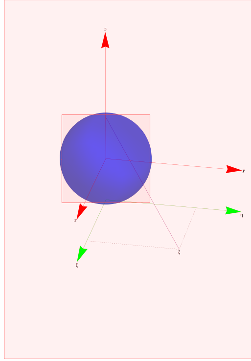
Figure 1.7. Stereographic projection of a point on a sphere.
