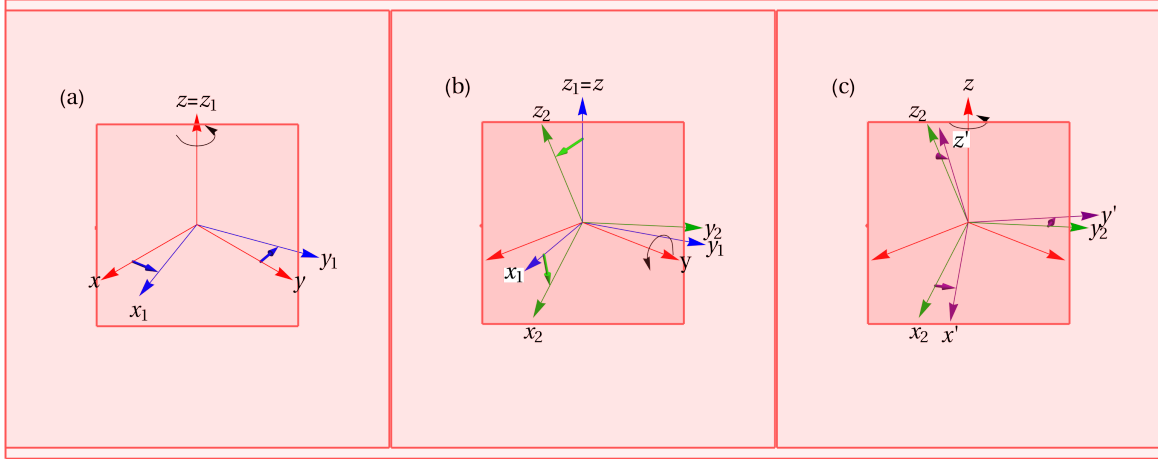
Figure 1.4. Succession of rotations of a coordinate system according to scheme B.
