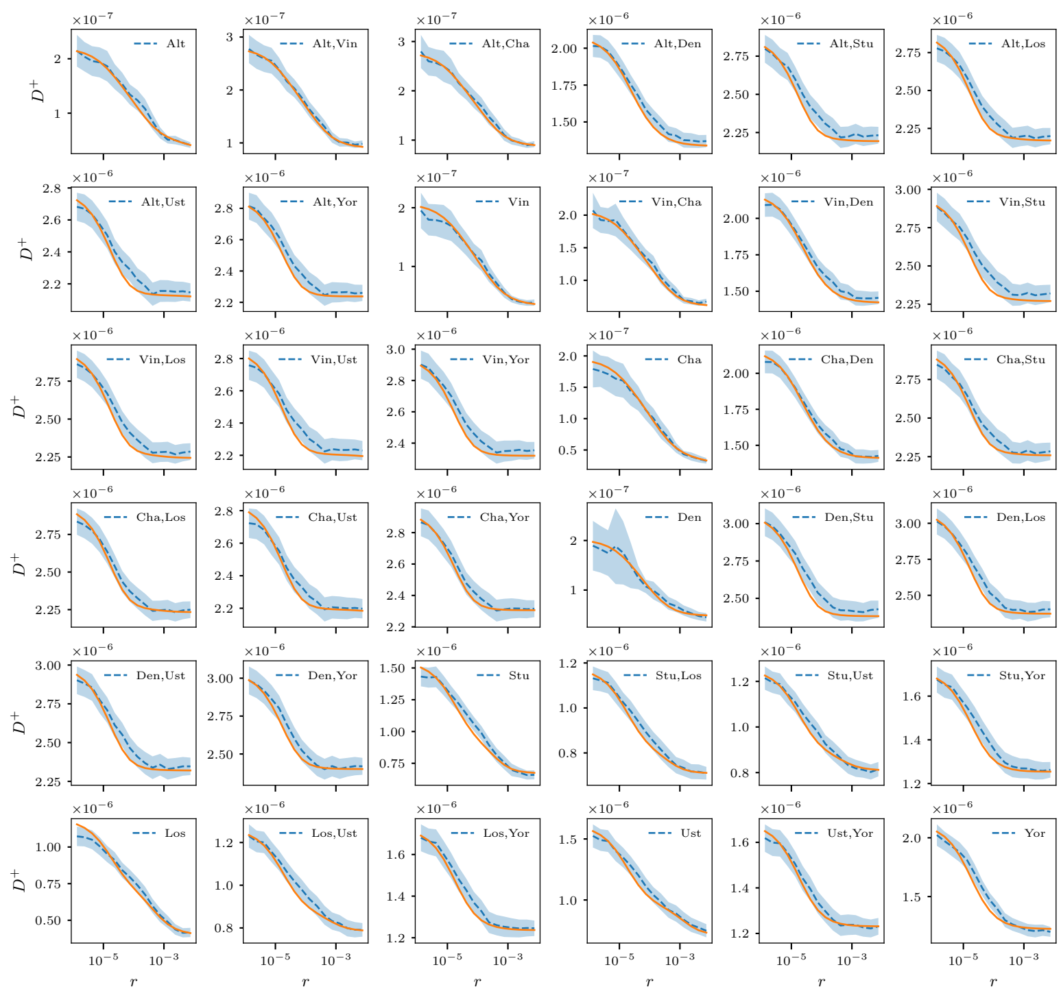
— Data (Zhou JHS map) — Full model
