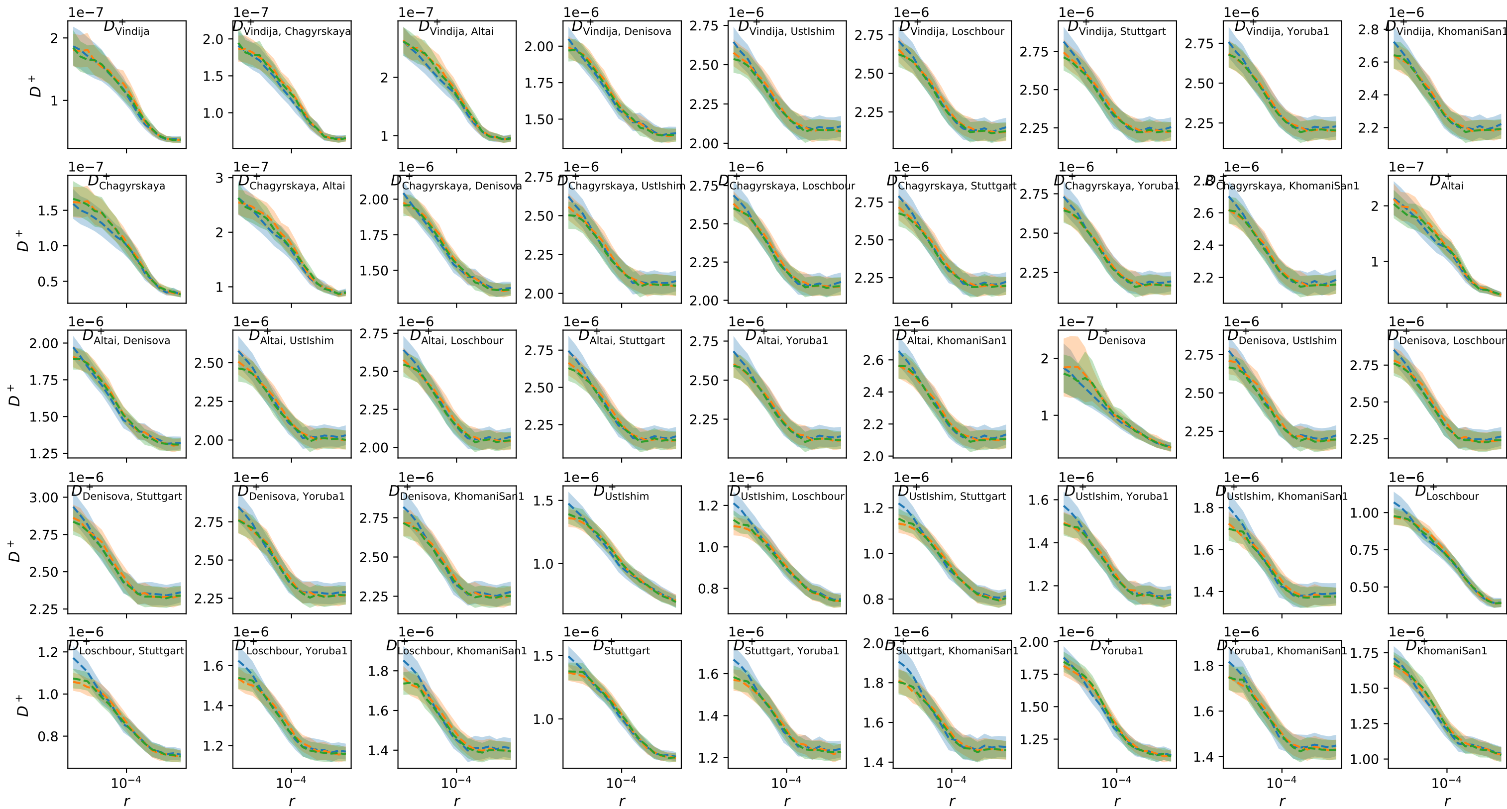
Empirical D^+ computed with Bherer, Zhou recombination maps
