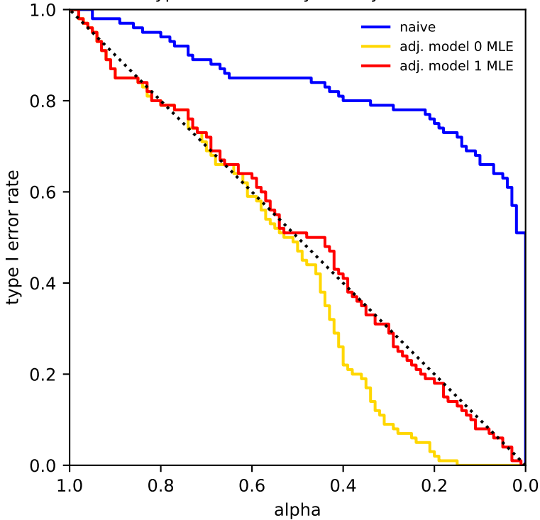
Type I error: Ne-asymmetry models
