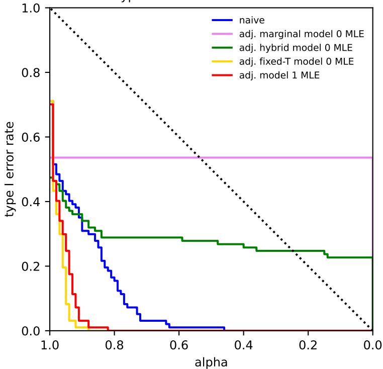
Type I error: contraction models
