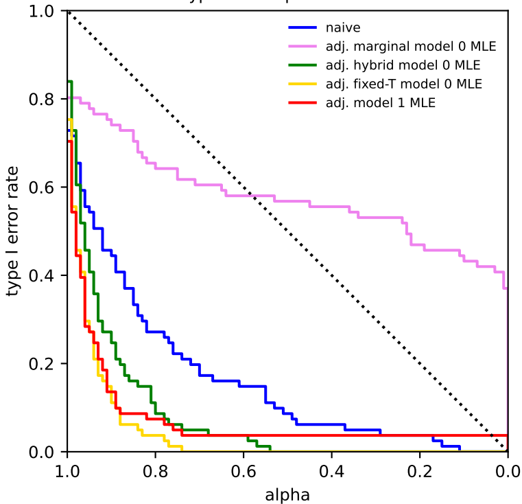
Type I error: pulse models
