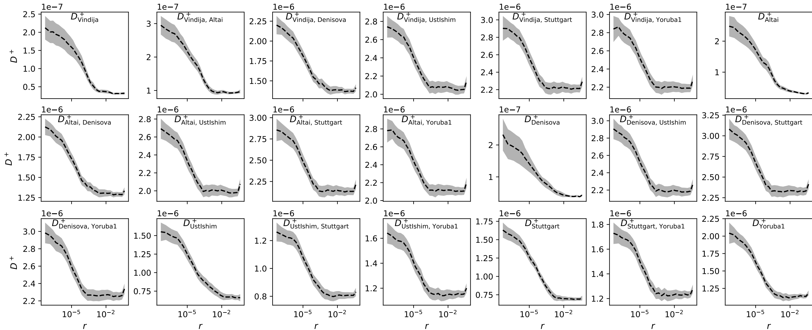
Empirical D^+ computed with Bherer recombination map
