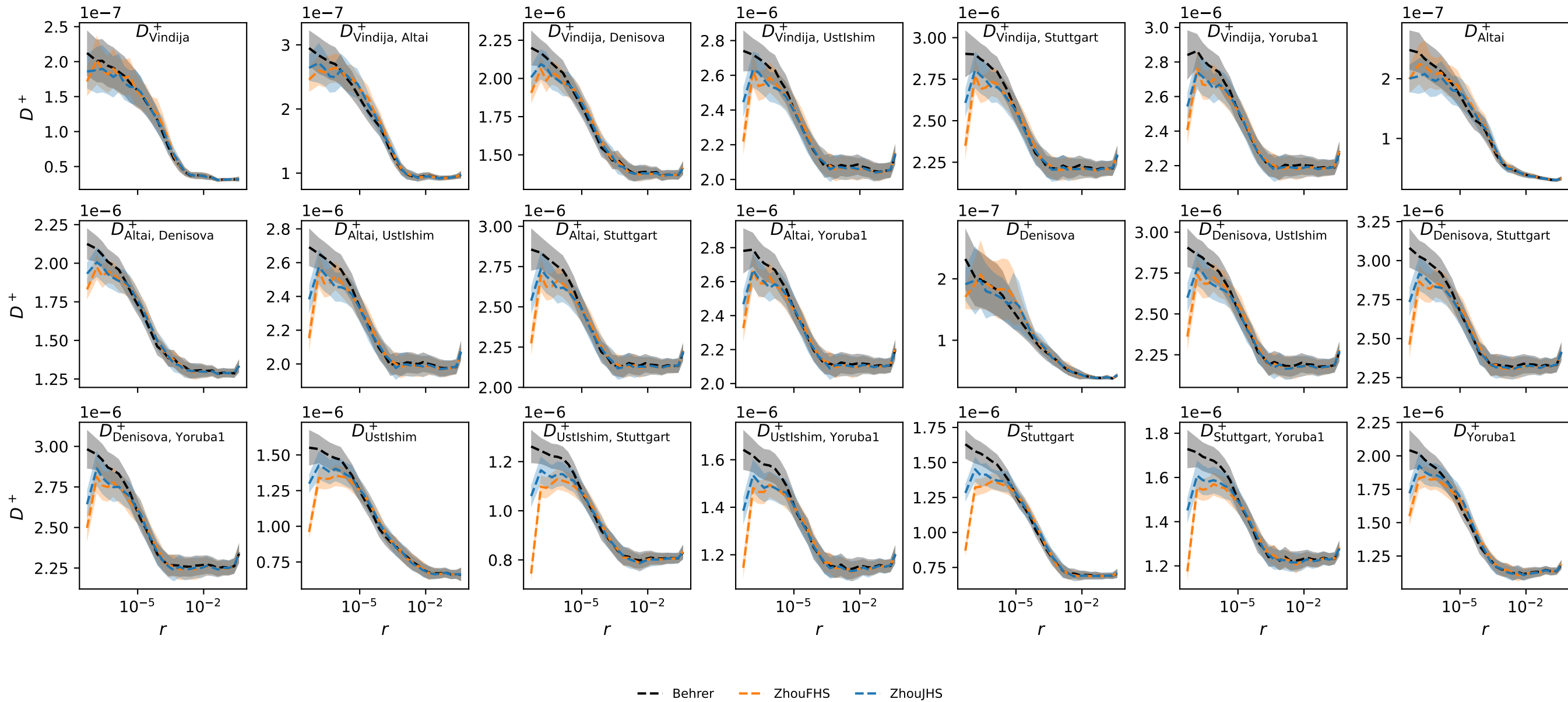
Empirical D^+ computed with 3 recombination maps
