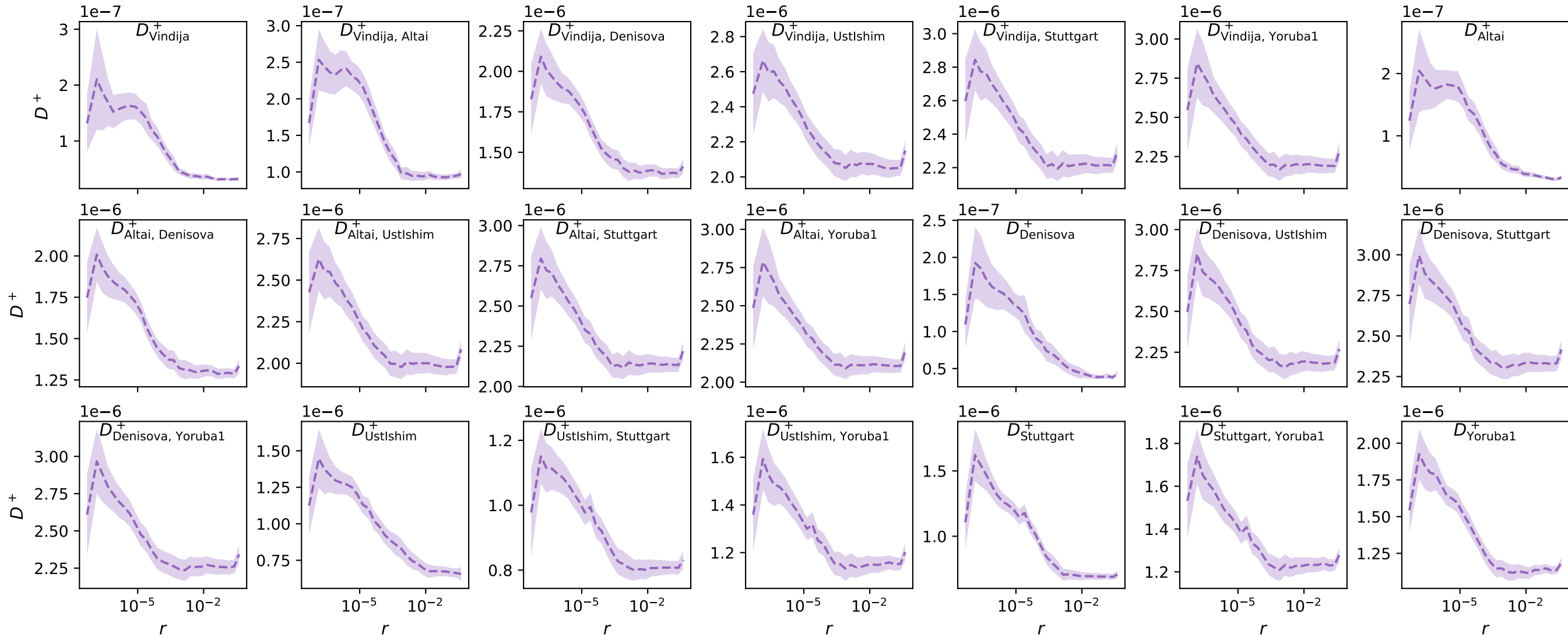
Empirical D^+ computed with omniFIN recombination map
