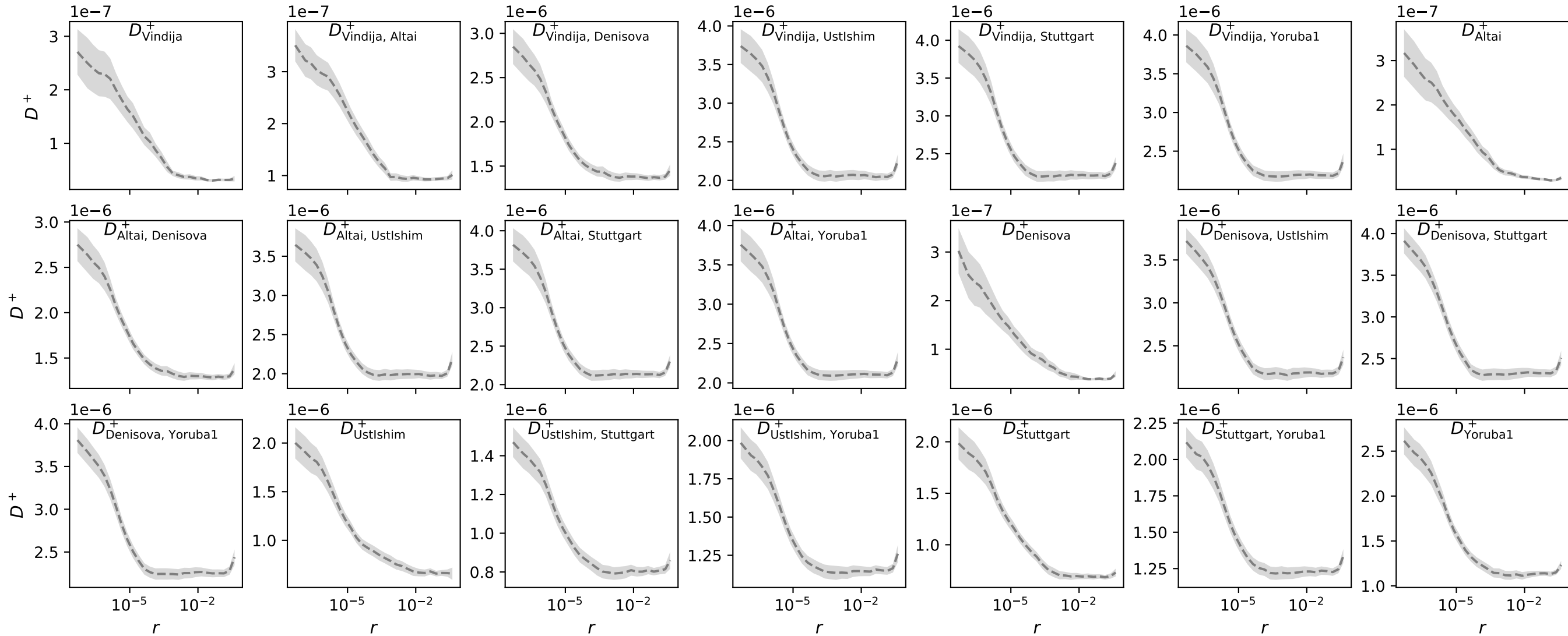
Empirical D^+ computed with pyrhoFIN recombination map
