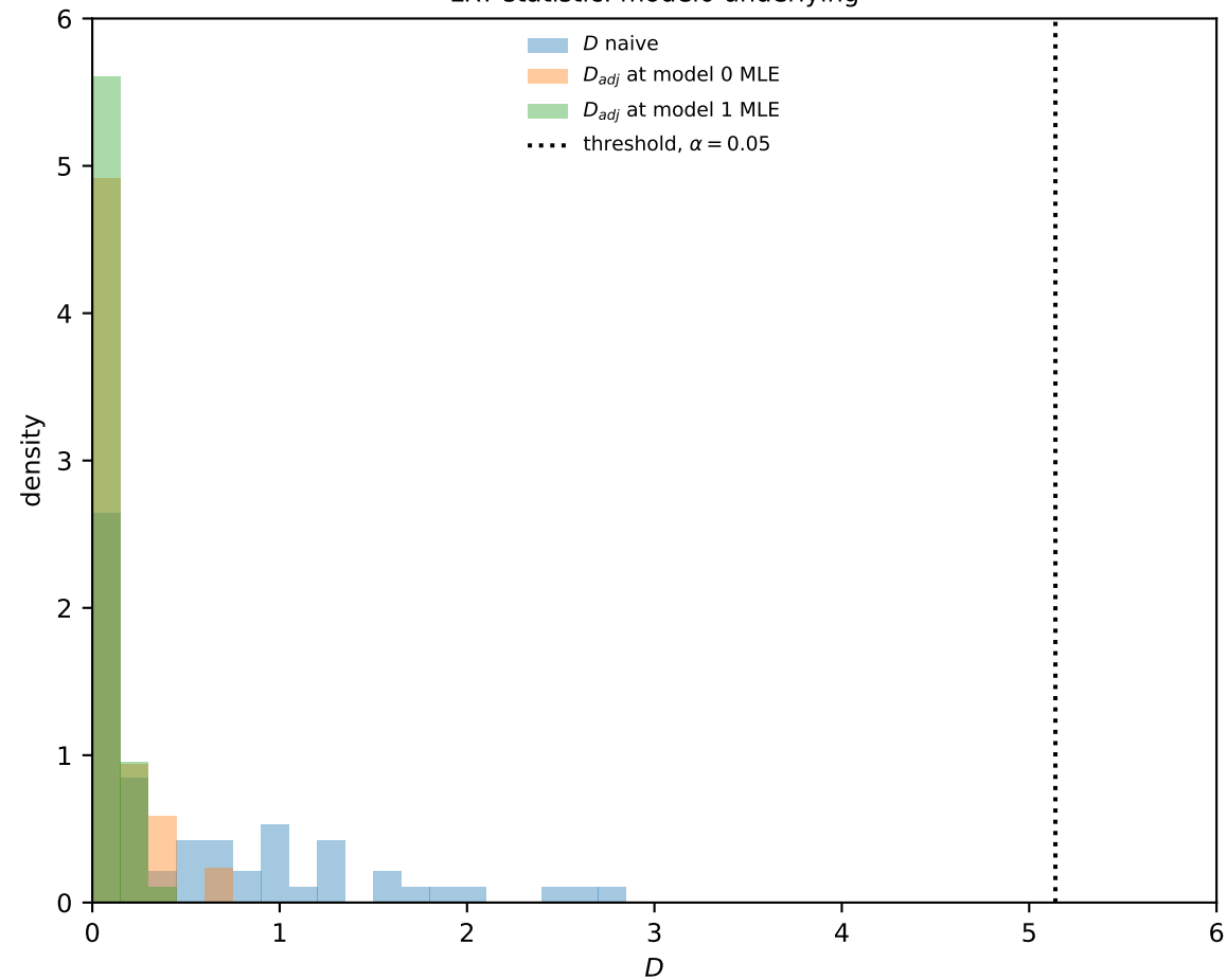
LRT statistic: model0 underlying
