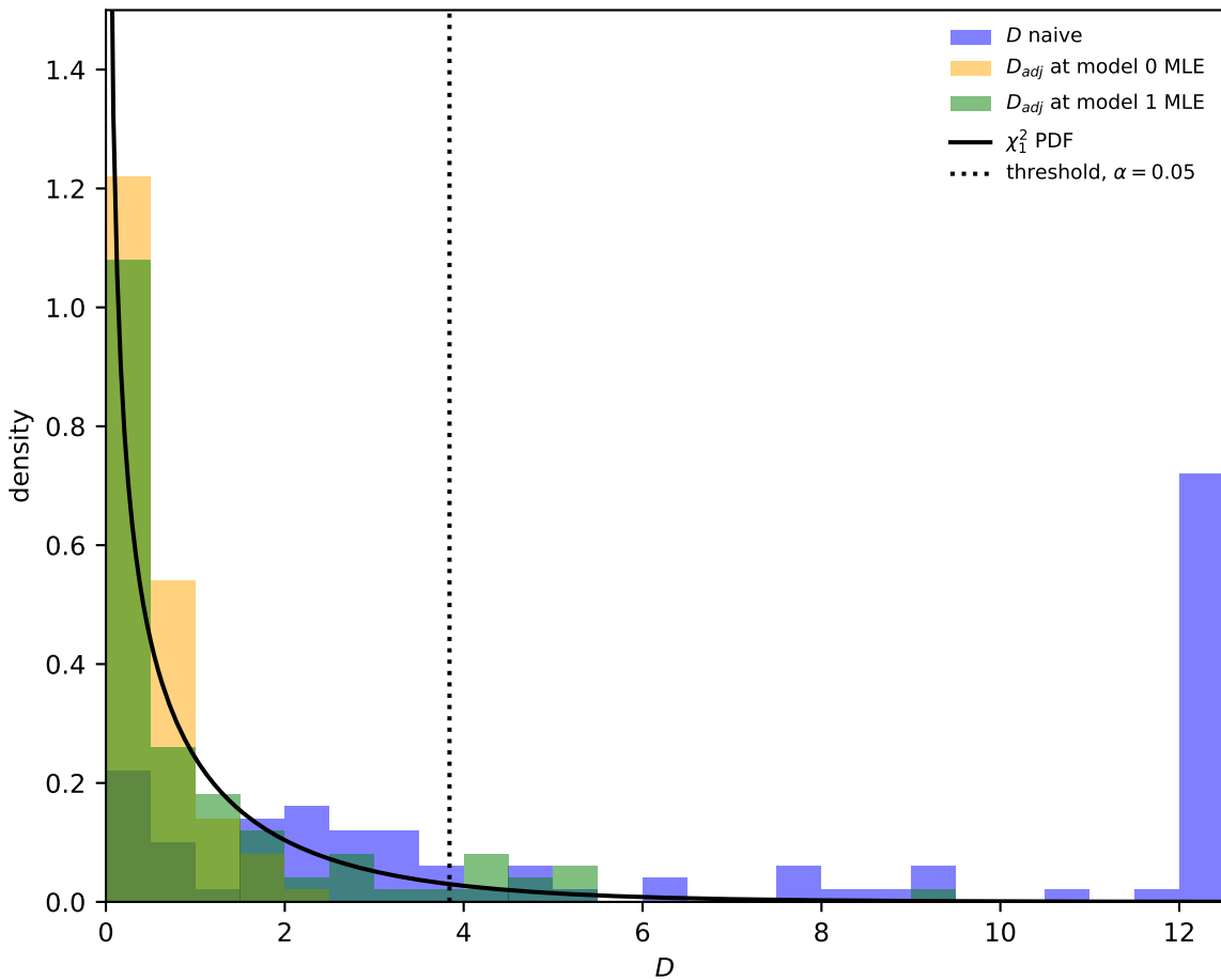
LRT statistic: model0 underlying
