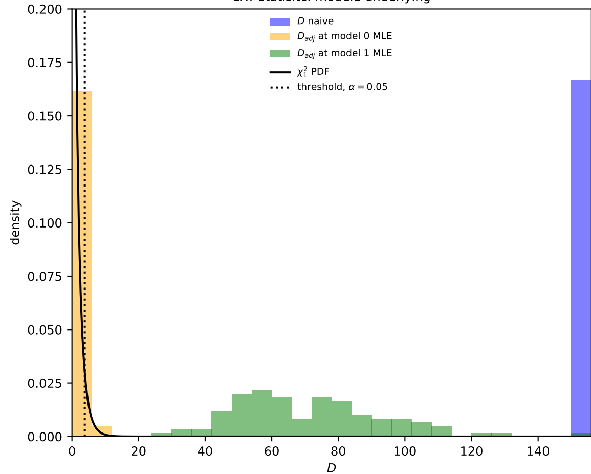
LRT statistic: model1 underlying
