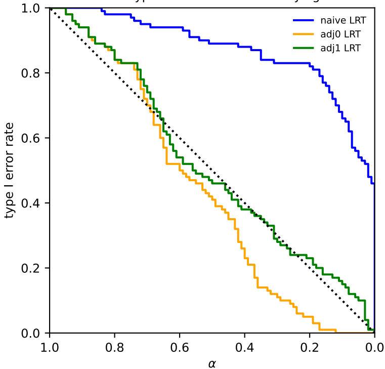
LRT type I error: model0 underlying
