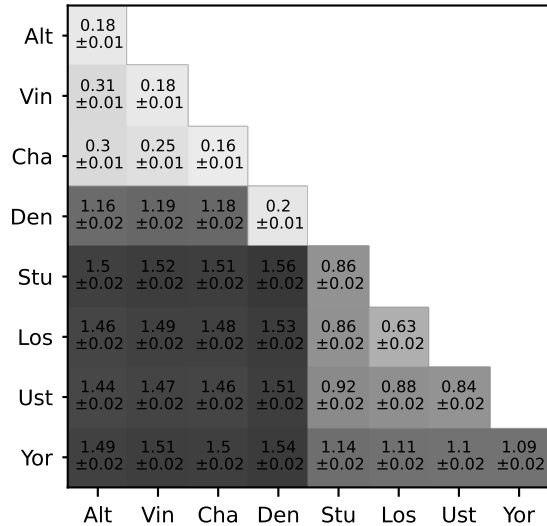
observed H
