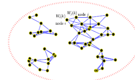
Fig. 1. A graphical illustration of the distributed learning problem over the time-varying undirected random network with 50 nodes in a time instant k , k \in \mathbb{N} , as an example. Each node i has its own raw dataset S_i = \{(x_i^t, y_i^t)\}_{t=1}^{N_i} , whose size is N_i . The locally blocked datasets S_i , i = 1, 2, \dots, N , compose the entire dataset S . In the learning process at each time instant k \in \mathbb{N} , only two neighboring nodes (e.g., node i and node j ) are randomly selected successively. Only the two selected nodes in the network have access to the output weight vectors (e.g., W_i(k) and W_j(k) ) from each other, and the other nodes stay silent and idle at the time instant. The goal of the problem is to obtain a global optimal output weight vector W^* only with the raw dataset that is distributed and blocked among the spatially distinct nodes in the network by using a gossip-based communication protocol.
