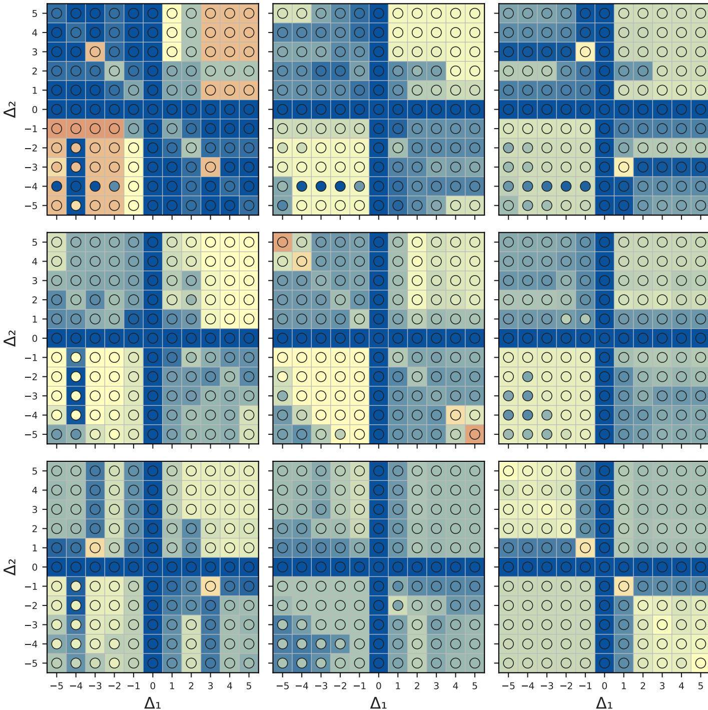
R 1 = mono (1-mer)
