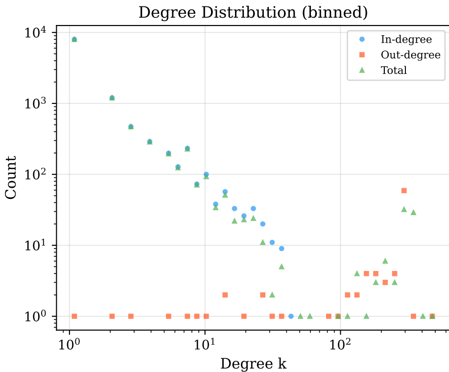
Figure 1: Simcluster Follow-Network Degree Distributions
