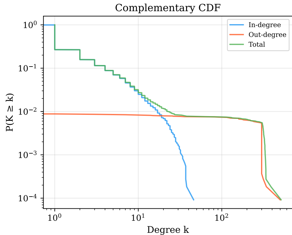
Figure 1: Simcluster Follow-Network Degree Distributions
