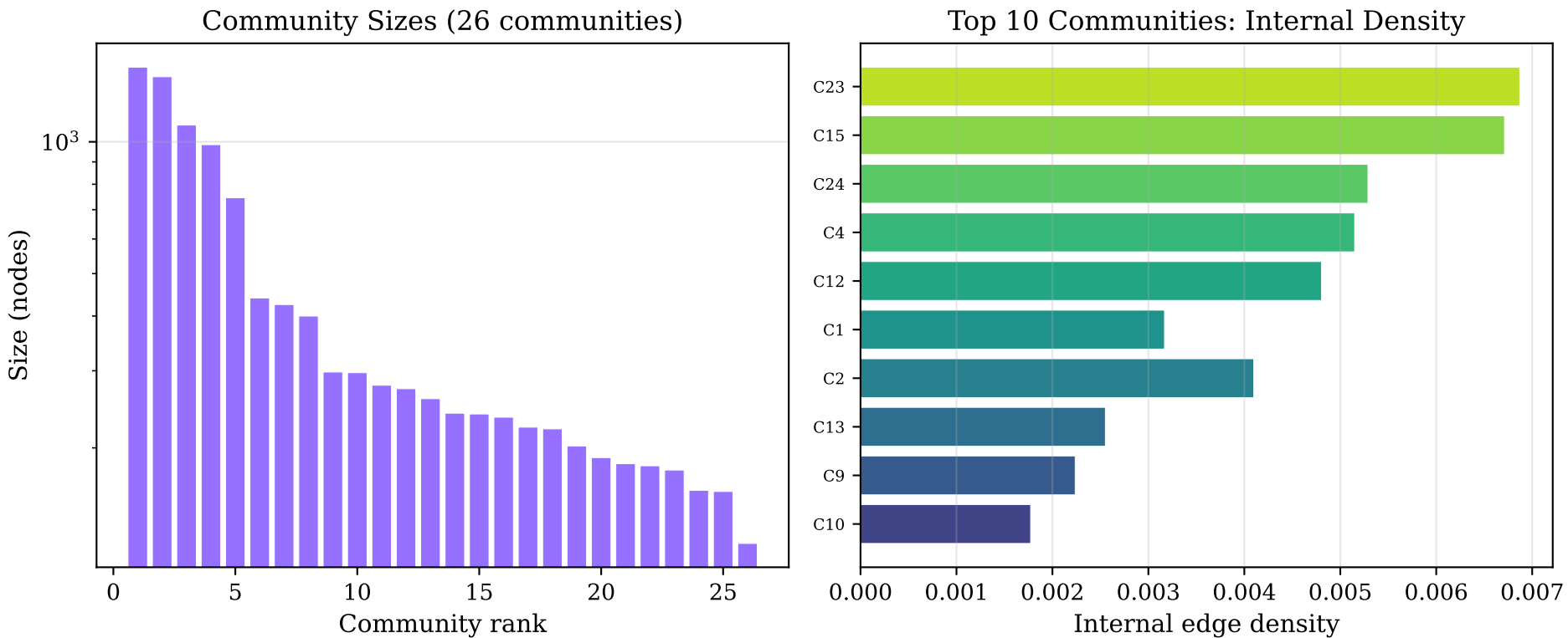
Figure 3: Louvain Community Detection (modularity=0.535)
