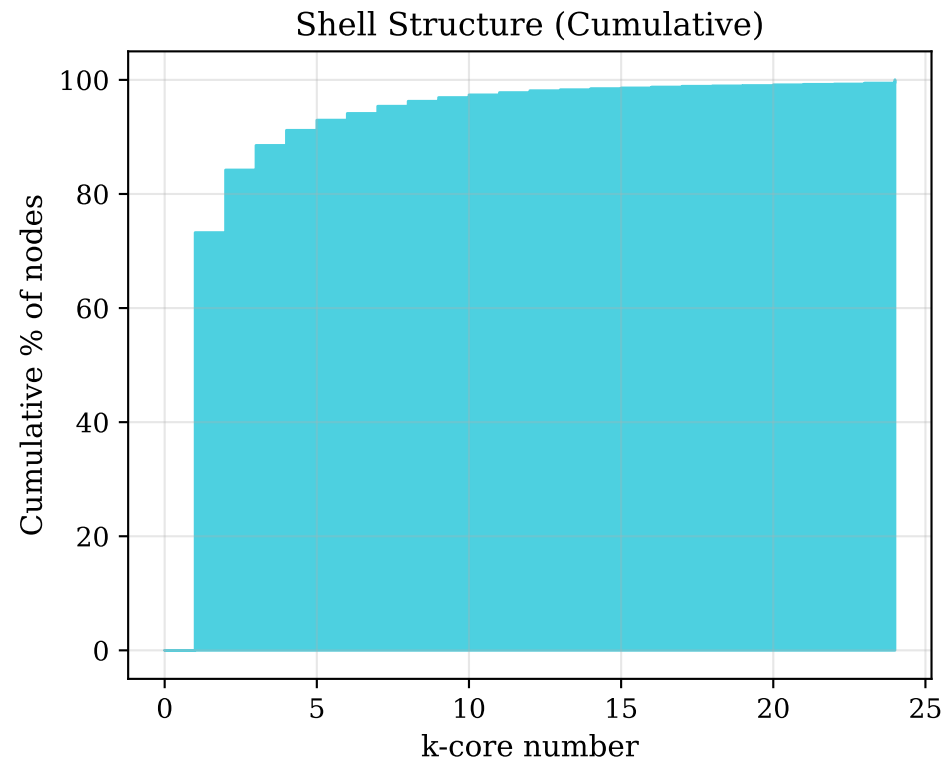
Figure 5: k-Core Decomposition
