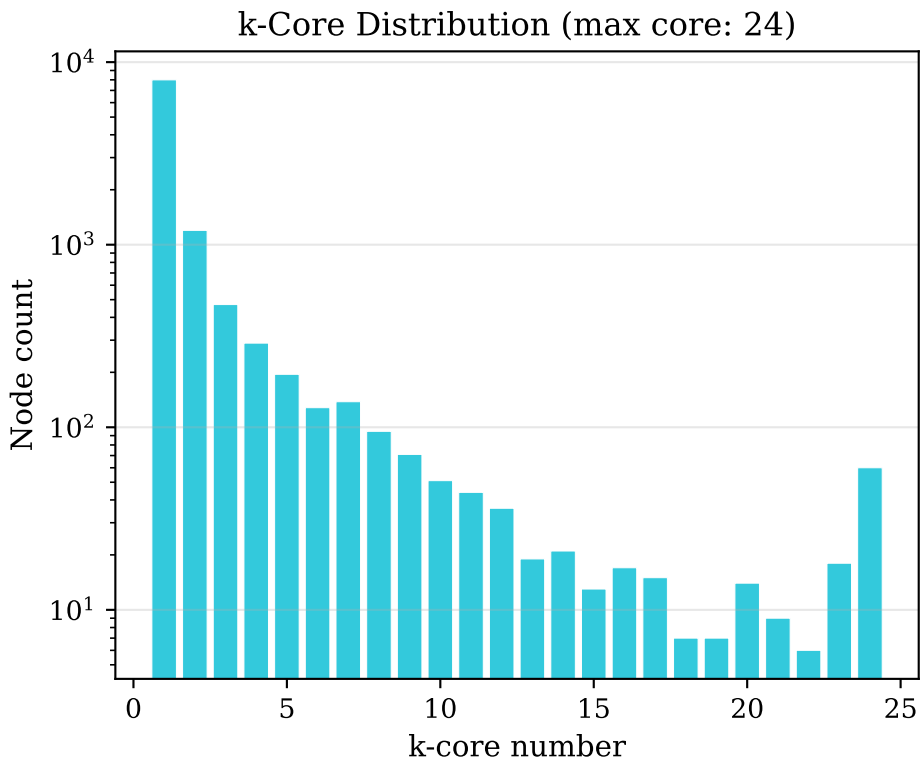
Figure 5: k-Core Decomposition
