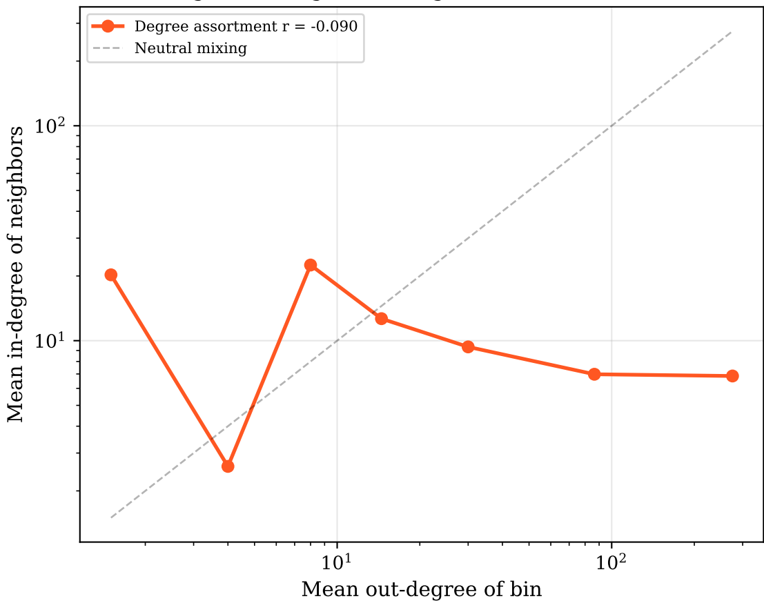
Figure 8: Degree Mixing Pattern ( r = -0.090 )
