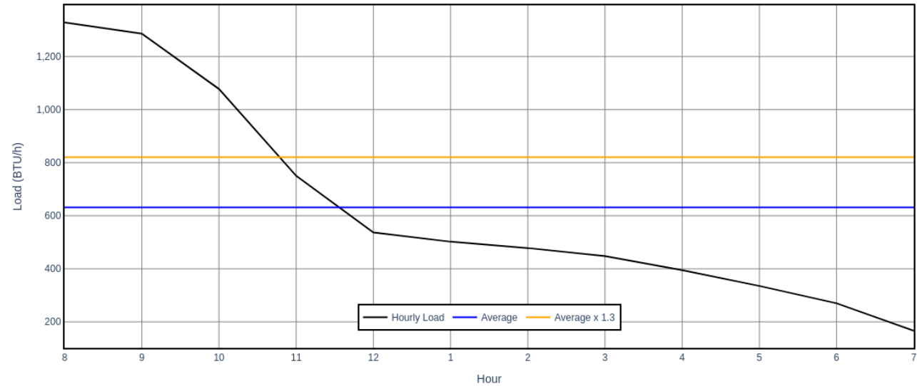
Kitchen (First) - Hourly Fenestration Load - Midsummer
