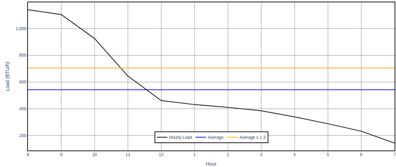
Bedroom 1 (First) - Hourly Fenestration Load - Midsummer
