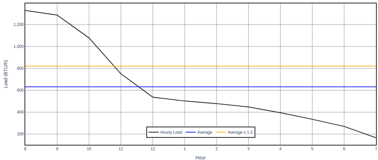
Kitchen (First) - Hourly Fenestration Load - Midsummer
