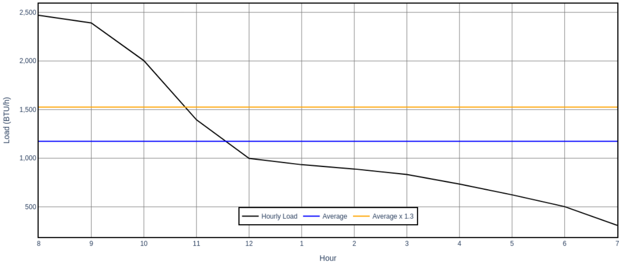
Zone 1 - Hourly Fenestration Load - Midsummer
