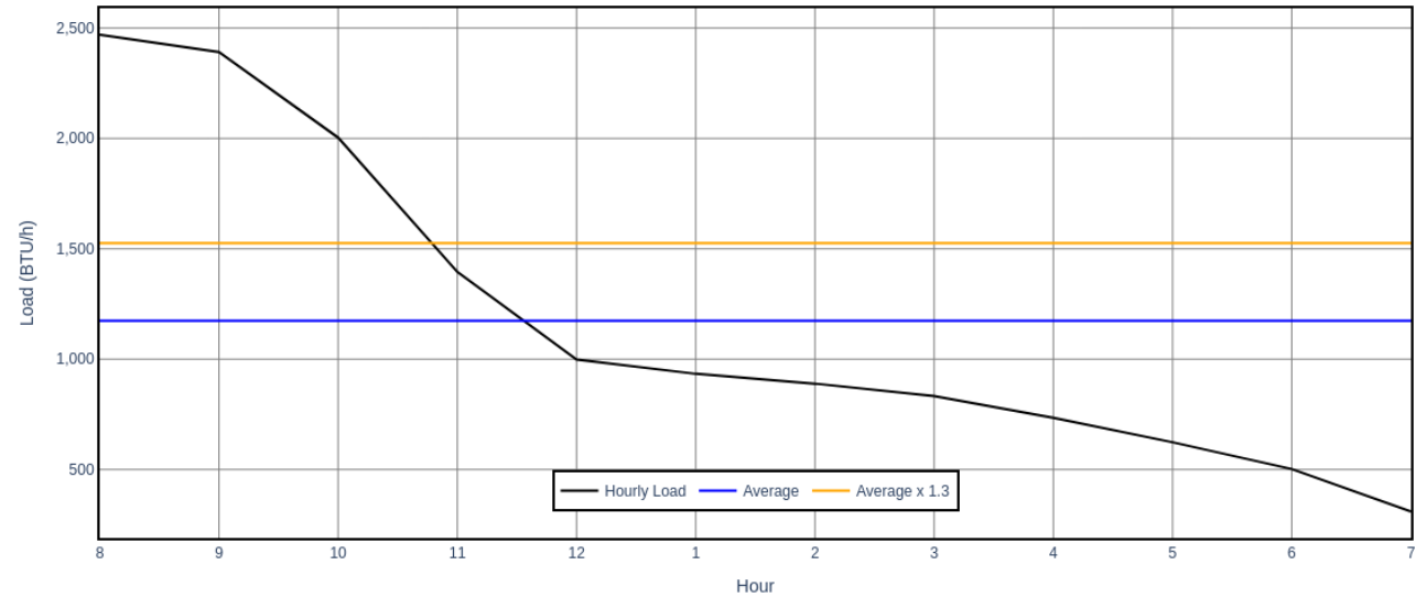
Zone 1 - Hourly Fenestration Load - Midsummer
