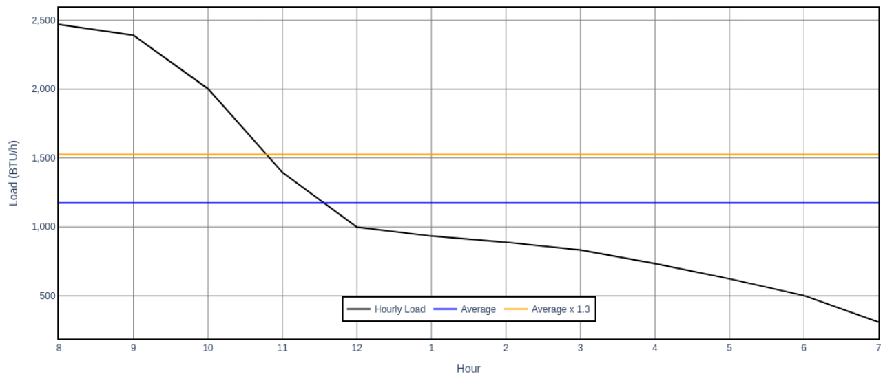
Cold Climate Heat Pump - Hourly Fenestration Load - Midsummer
