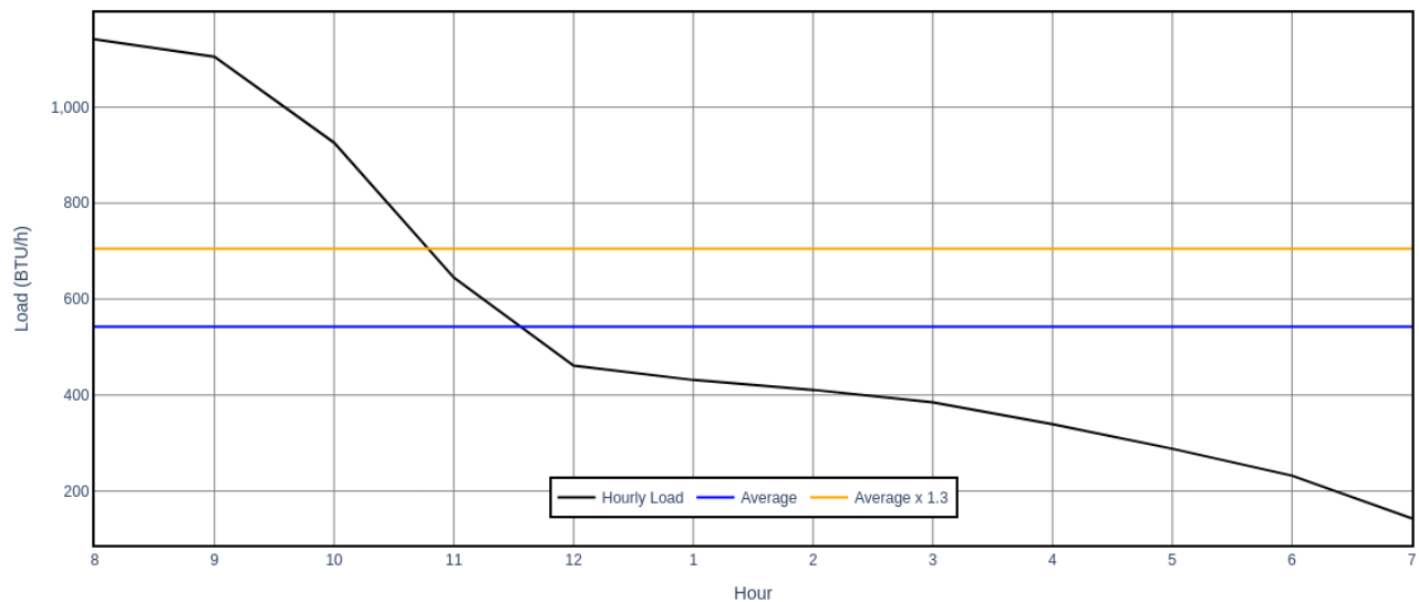
Bedroom 1 (First) - Hourly Fenestration Load - Midsummer
