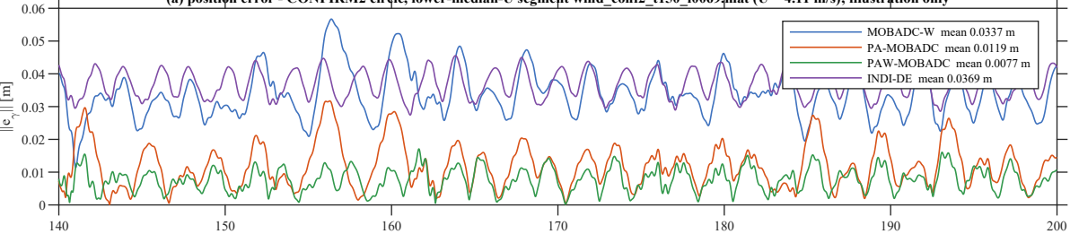
(a) position error - CONFIRM2 circle, lower-median-U segment wind_conf2_t150_i0069.mat (U = 4.11 m/s); illustration only
