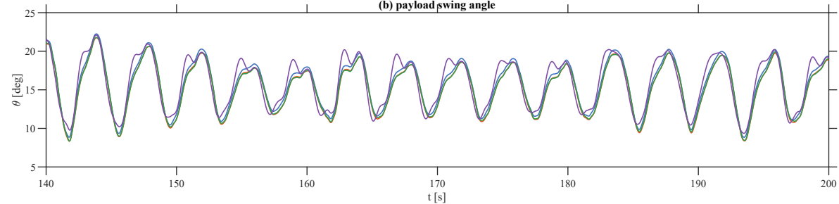
(b) payload swing angle
