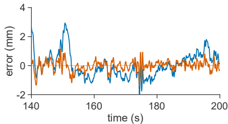
f hover: tracking error north
