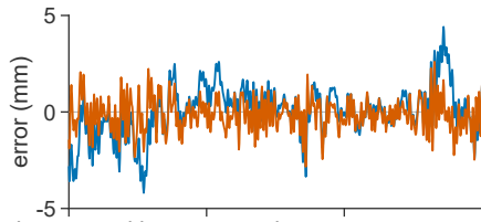
f hover: tracking error north
