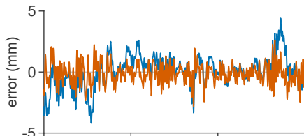
f hover: tracking error north
