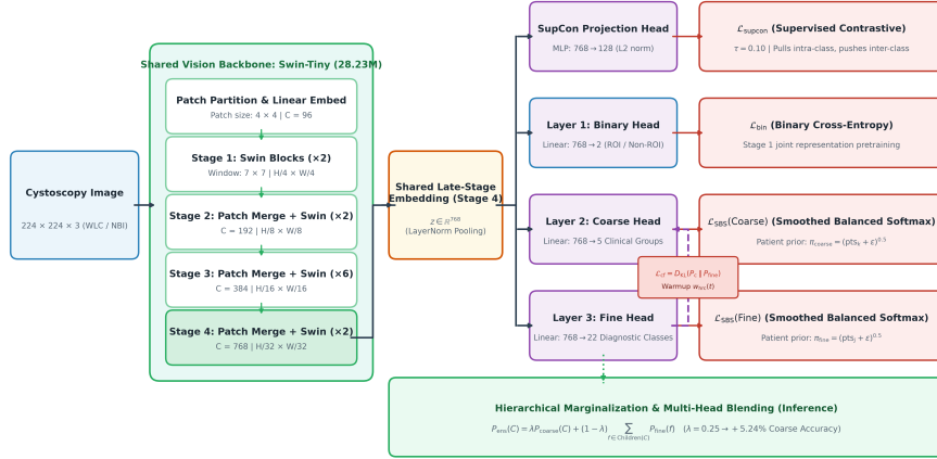
Fig. 2. Architecture and workflow of the proposed CystoHier framework: Endoscopy images are processed through a shared Swin-Tiny backbone. Features z \in \mathbb{R}^{768} are classified via three hierarchical heads, supervised by Supervised Contrastive Loss ( \mathcal{L}_{\text{supcon}} ), task losses ( \mathcal{L}_{\text{bin}} , \mathcal{L}_{\text{SBS}}(\text{coarse}) , \mathcal{L}_{\text{SBS}}(\text{fine}) ) with Patient-Count Priors, and Coarse-Fine Consistency ( \mathcal{L}_{\text{cf}} ) with Curriculum Warmup scheduling.
