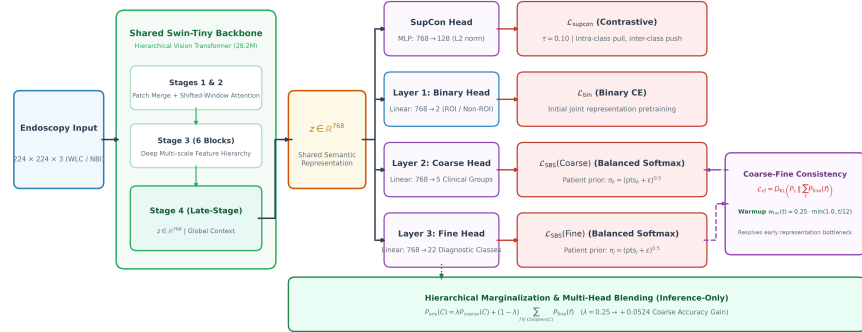
Fig. 2. Architecture and workflow of the proposed CystoHier framework: Endoscopy images are processed through a shared Swin-Tiny backbone. Features z \in \mathbb{R}^{768} are classified via three hierarchical heads, supervised by Supervised Contrastive Loss ( \mathcal{L}_{\text{supcon}} ), task losses ( \mathcal{L}_{\text{bin}} , \mathcal{L}_{\text{SBS}} (coarse), \mathcal{L}_{\text{SBS}} (fine)) with Patient-Count Priors, and Coarse-Fine Consistency ( \mathcal{L}_{\text{cf}} ) with Curriculum Warmup scheduling.
