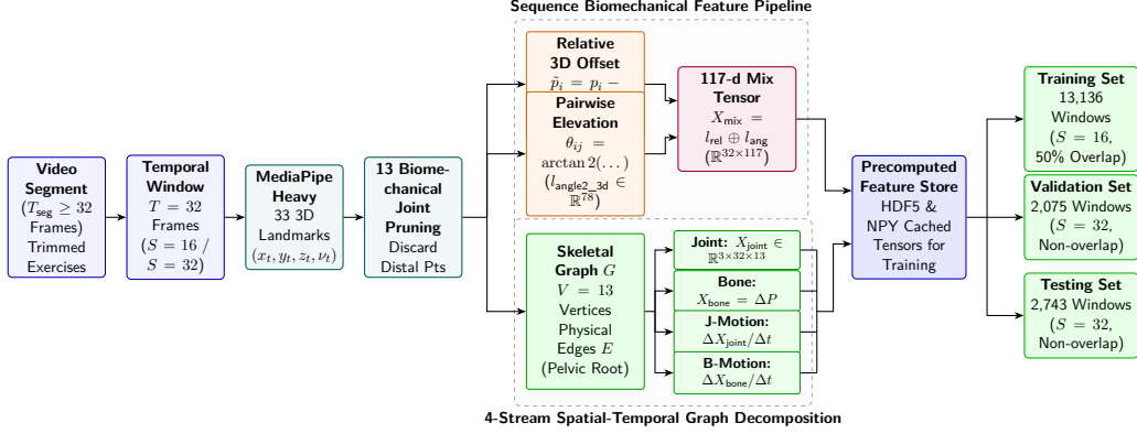
Figure 4: The proposed Biomechanical Feature Extraction and Kinematic Tensor Decomposition pipeline: illustrating the two-branch extraction of the 117-d sequence mix and the 4-stream spatial-temporal graph tensors.
