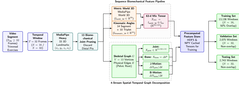
Fig. 4: The proposed Biomechanical Feature Extraction and Kinematic Tensor Decomposition pipeline: illustrating the two-branch extraction of the 63-d sequence mix and the 4-stream spatial-temporal graph tensors.
