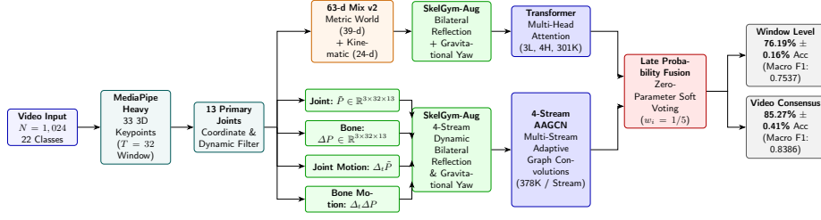
Fig. 1: The proposed SkelGym architecture: an end-to-end cross-paradigm framework coupling self-attention sequence modeling with multi-stream adaptive graph convolutional networks via zero-parameter uniform average soft voting.
