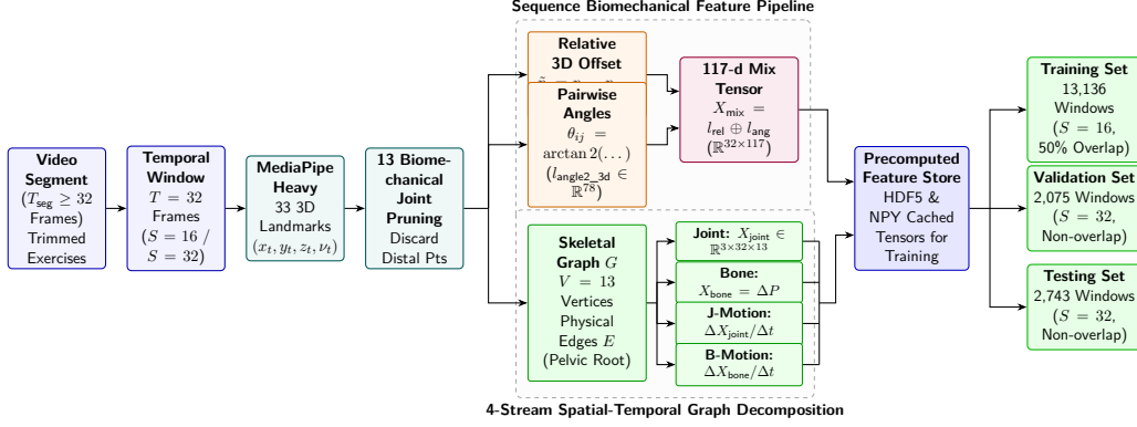
Figure 4: The proposed Biomechanical Feature Extraction and Kinematic Tensor Decomposition pipeline: illustrating the two-branch extraction of the 117-d sequence mix and the 4-stream spatial-temporal graph tensors.
