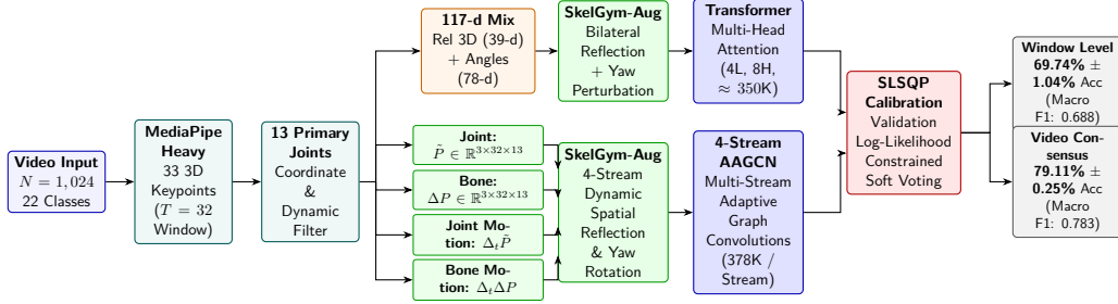
Figure 1: The proposed SkelGym architecture: an end-to-end cross-paradigm framework coupling self-attention sequence modeling with multi-stream adaptive graph convolutional networks via validation-calibrated weighted soft voting.
